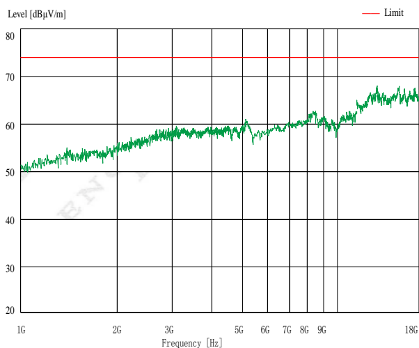
Antenna Horizontal
