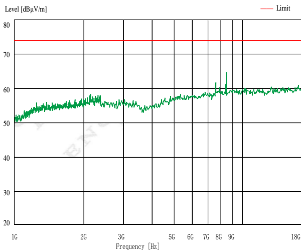
Antenna Vertical
