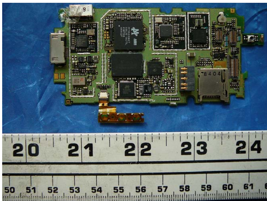
EUT – Main Board Top View without Shielding
