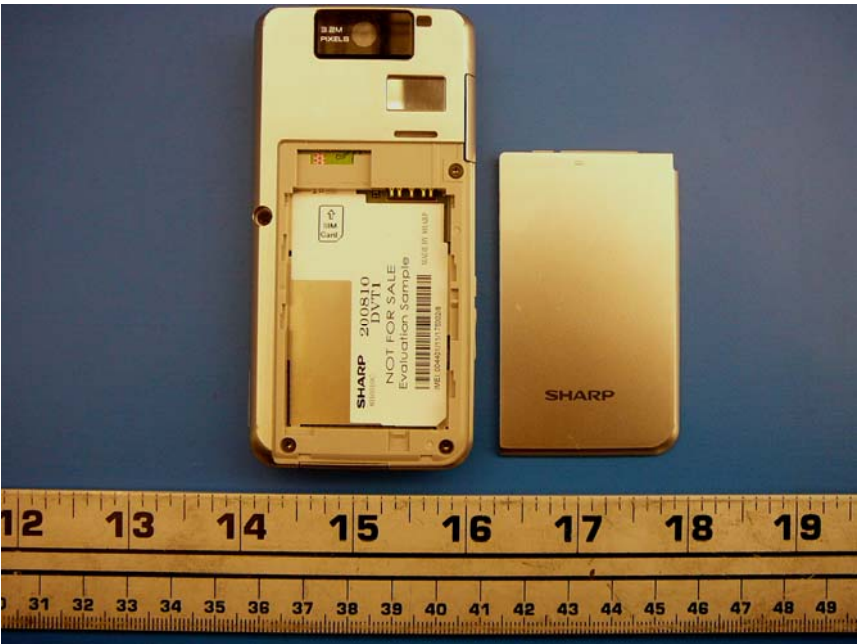
EUT – Uncovered View with Battery
