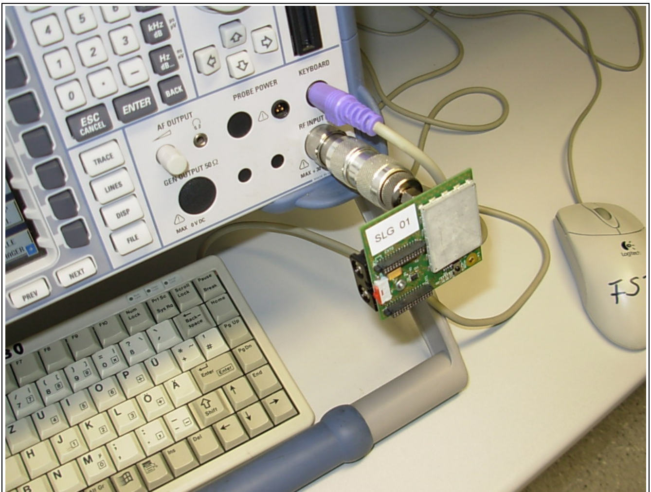
Figure 1: Measurement set-up for conducted measurement acc. to following sections of the report 1228-09-EE-10-PB005: 4.1.1; 4.1.2; 4.2; 4.3 and 4.4.3
