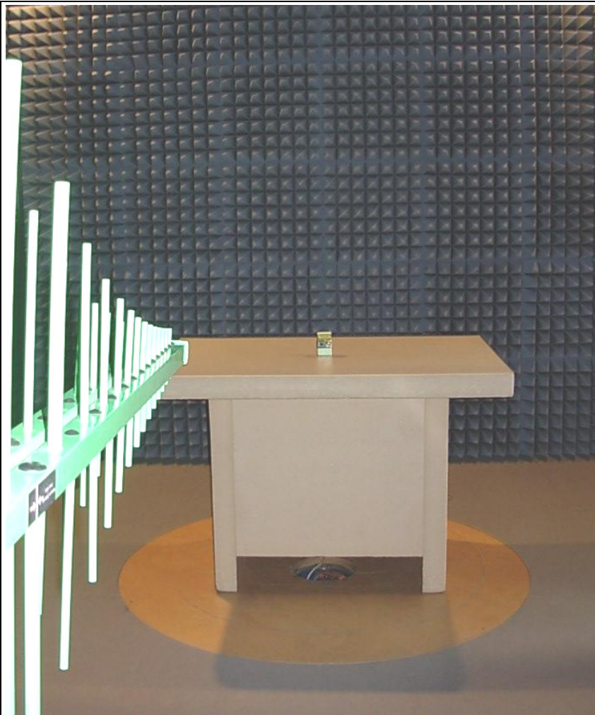
Figure 2: Measurement set-up for radiated measurement < 1 GHz acc. following sections of the report 1228-09-EE-10-PB005: 4.4.1 and 4.5.1
