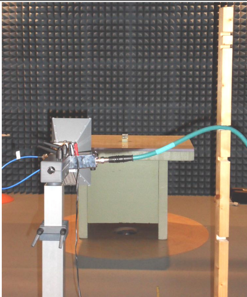
Figure 3: Measurement set-up for radiated measurement > 1 GHz acc. following sections of the report 1228-09-EE-10-PB005: 4.4.2 and 4.5.2
