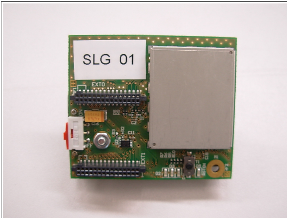
Figure 5: Plan view of EUT (acc. Test report 1228-09-EE-10-PB005)
