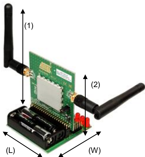
Figure 6-1. REB233CBB Module with vertical (1) and horizontal (2) antenna position
