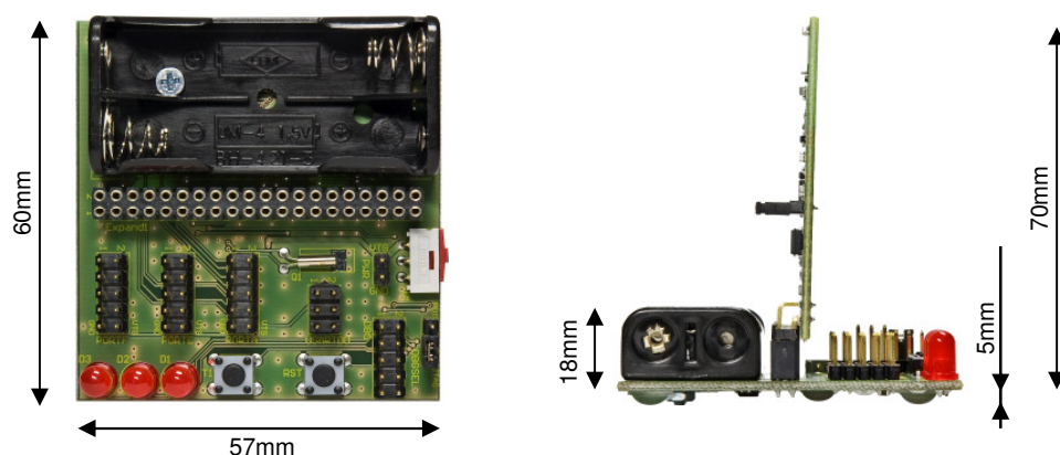
Figure 4-1. Mechanical outline.
