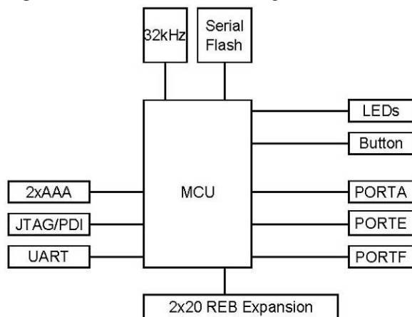
Figure 5-1. REB-CBB block diagram.
