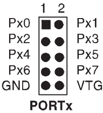
Figure 5-5. General pin-out of I/O port headers.
