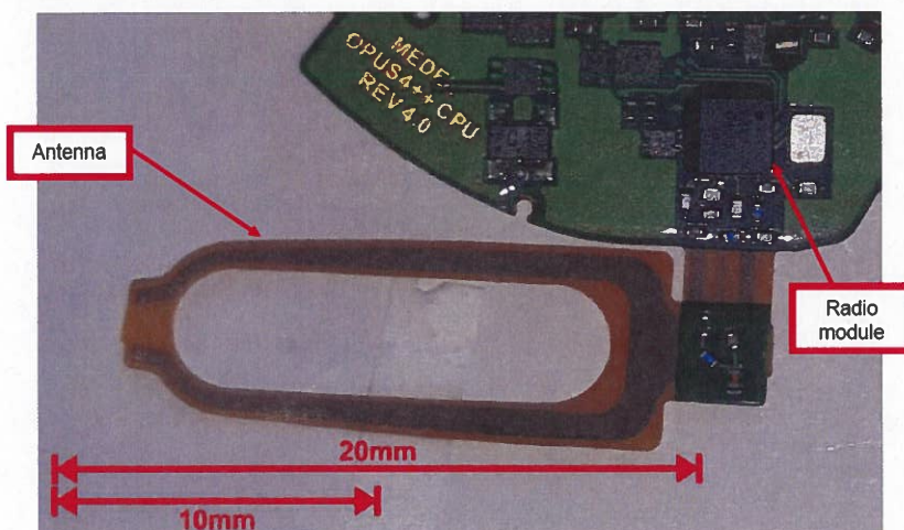
Fig. 1 Antenna and radio module
