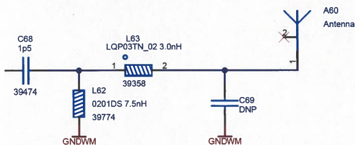
Fig. 2 Antenna impedance matching
