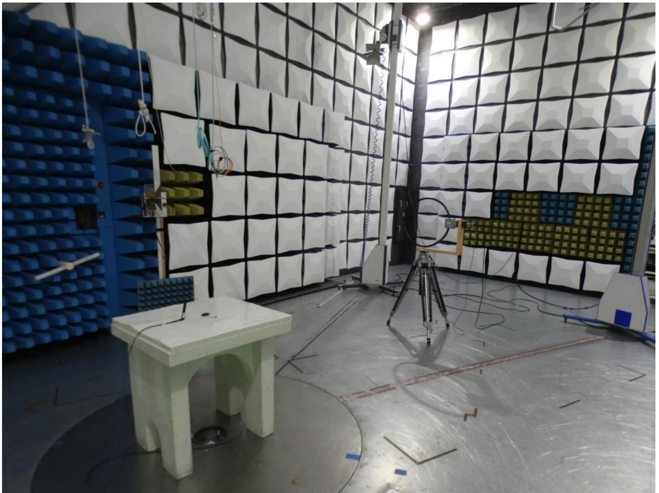
Photo 3: Test setup for radiated measurements (stand alone setup, 9 kHz - 30 MHz; FCC 15c247, ANSI 63.10)
