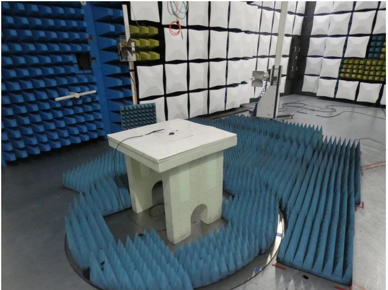
Photo 2: Test setup for radiated measurements (stand alone, semi-anechoic chamber above 1 GHz; unintentional radiator §15.109, ANSI C63.4)
