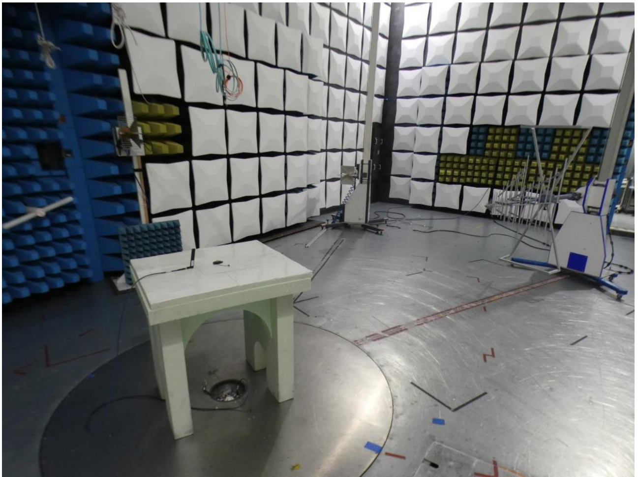
Photo 4: Test setup for radiated measurements (stand alone setup, 30 MHz - 1 GHz; FCC 15c247, ANSI 63.10)
