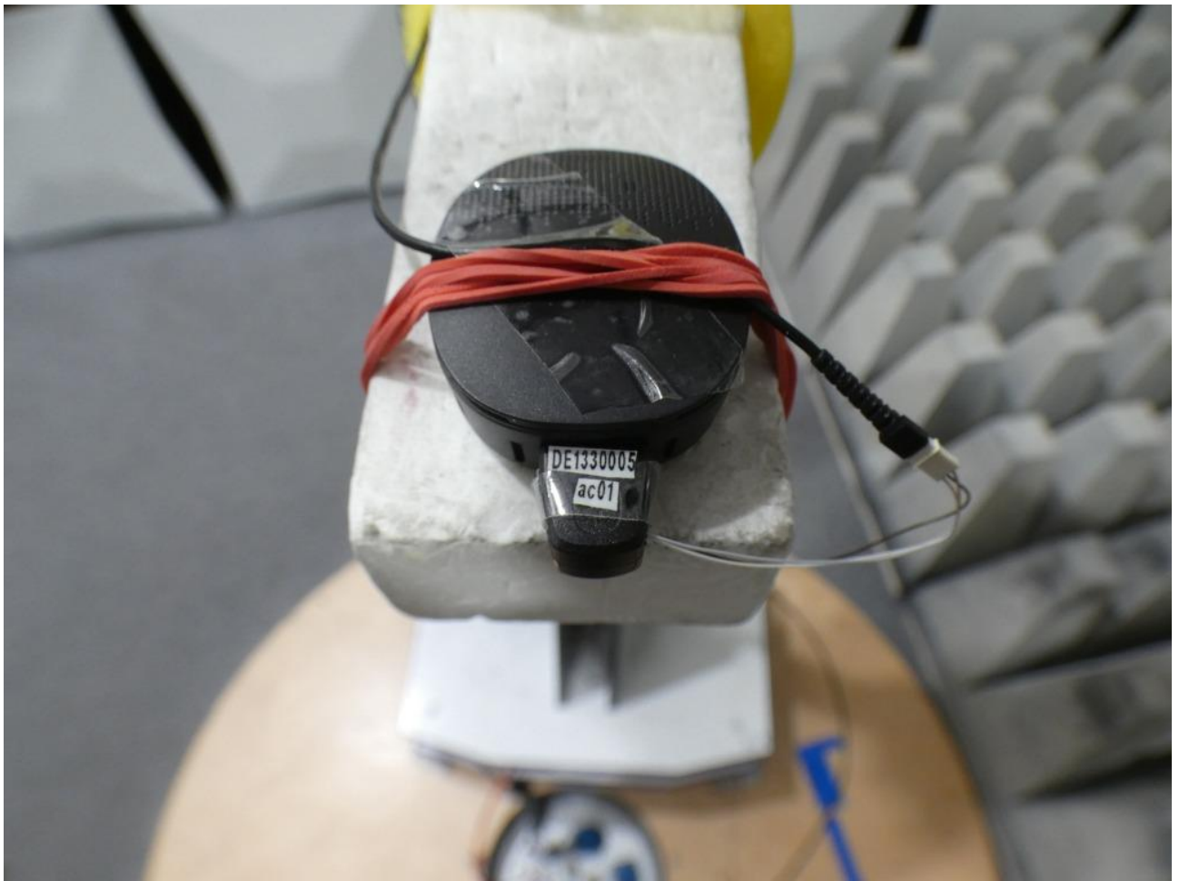
Photo 6: Test Setup for radiated measurements
