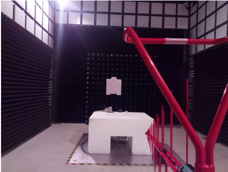
Radiated Emissions View - Front View (Below 1 GHz)
