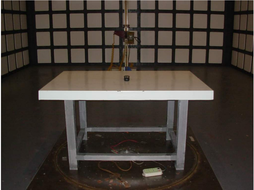
FRONT VIEW OF TEST (LYING, HIGH FREQUENCY)
