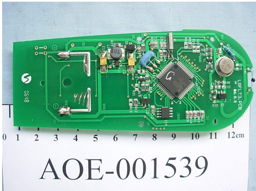
FIGURE 3 FIREPLACE REMOTE CONTROL SYSTEM (M/N: LGT202TX) MAIN BOARD (COMPONENT SIDE)
