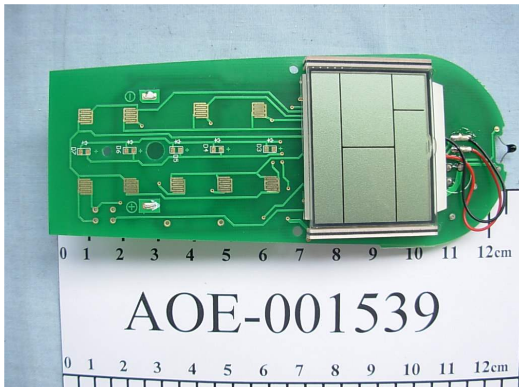
FIGURE 4 FIREPLACE REMOTE CONTROL SYSTEM (M/N: LGT202TX) MAIN BOARD (SOLDERED SIDE)
