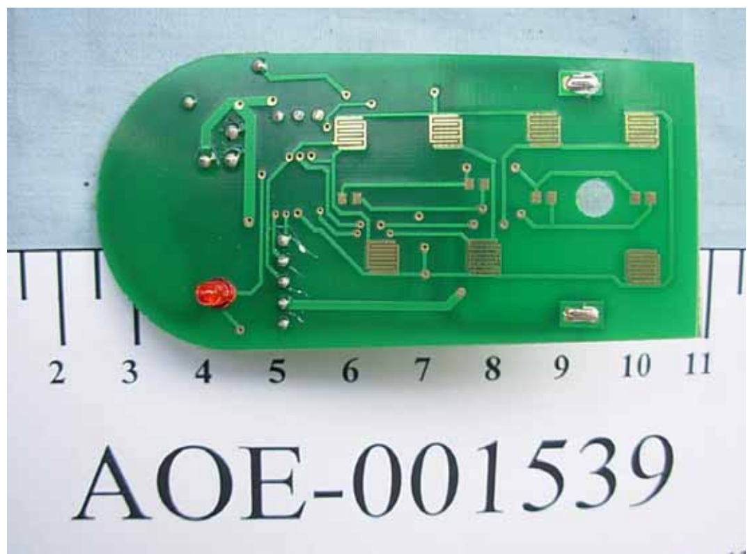
FIGURE 4 FIREPLACE REMOTE CONTROL SYSTEM (M/N: LGT201TX) MAIN BOARD (SOLDERED SIDE)
