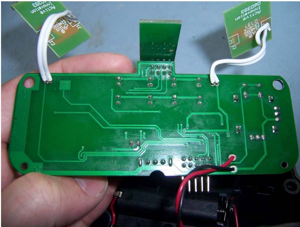
RemoteMainBoardBack
