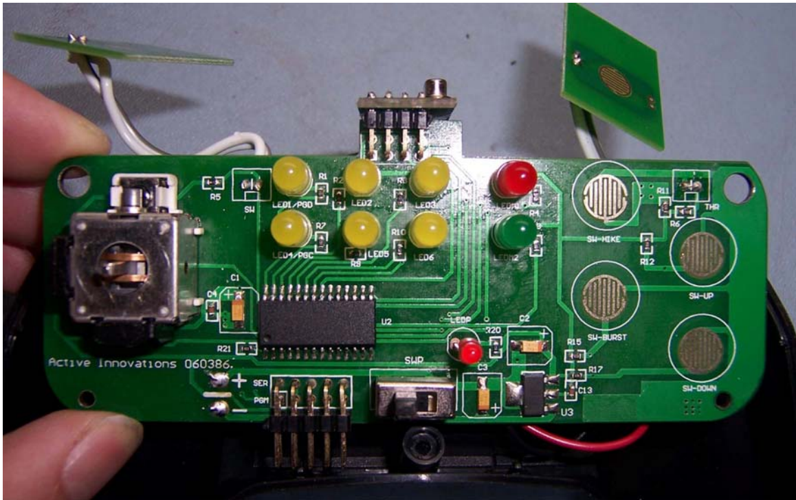
RemoteMainBoardFront
