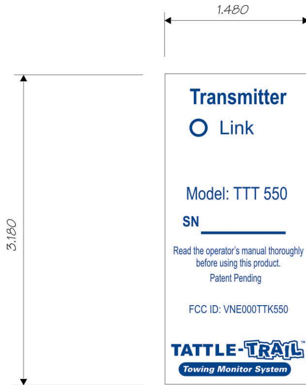
Transmitter Front 550-0007
