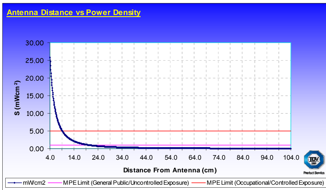
Figure 2 - This graph shows the S field (mW/cm²) strength value with regards to distance from the Antenna (cm)
