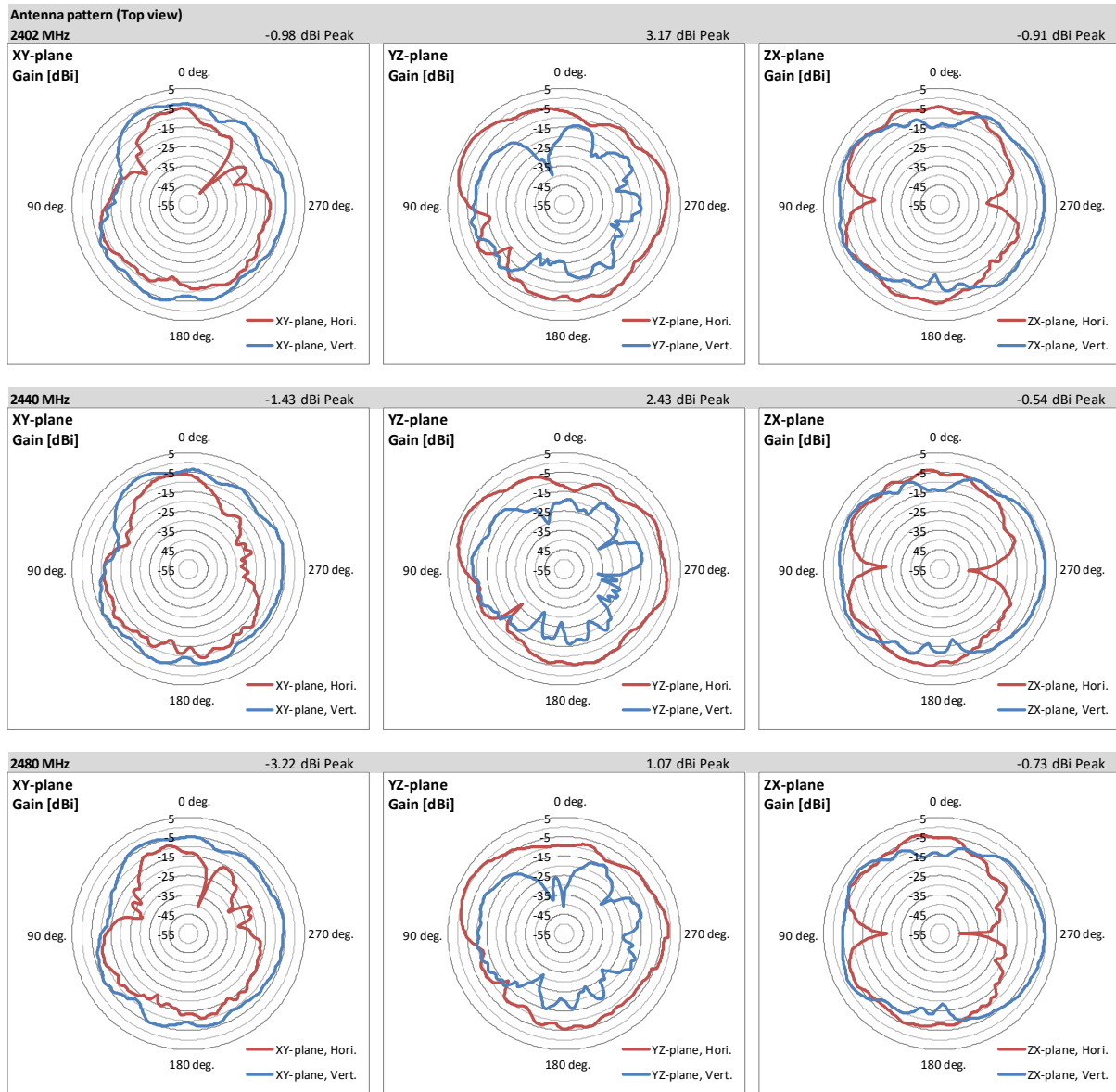
Antenna gain [UNIT: dBi]
