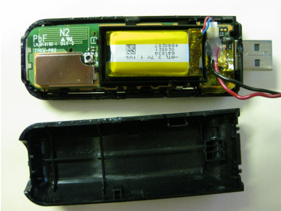
EUT with back cove removed
