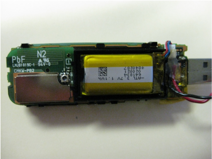
EUT with back cove removed
