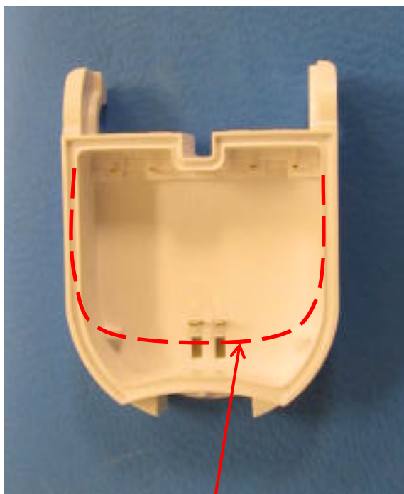
Antenna, molded into walls of plastic housing
