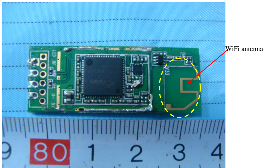
EUT – WiFi Module Top Components View
