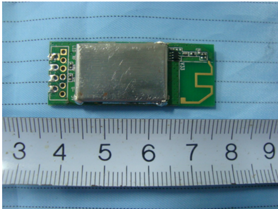
EUT – WiFi Module Top Components View
