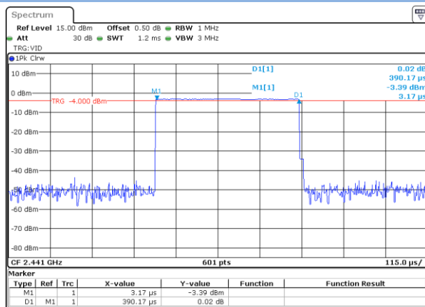
GFSK DH1
