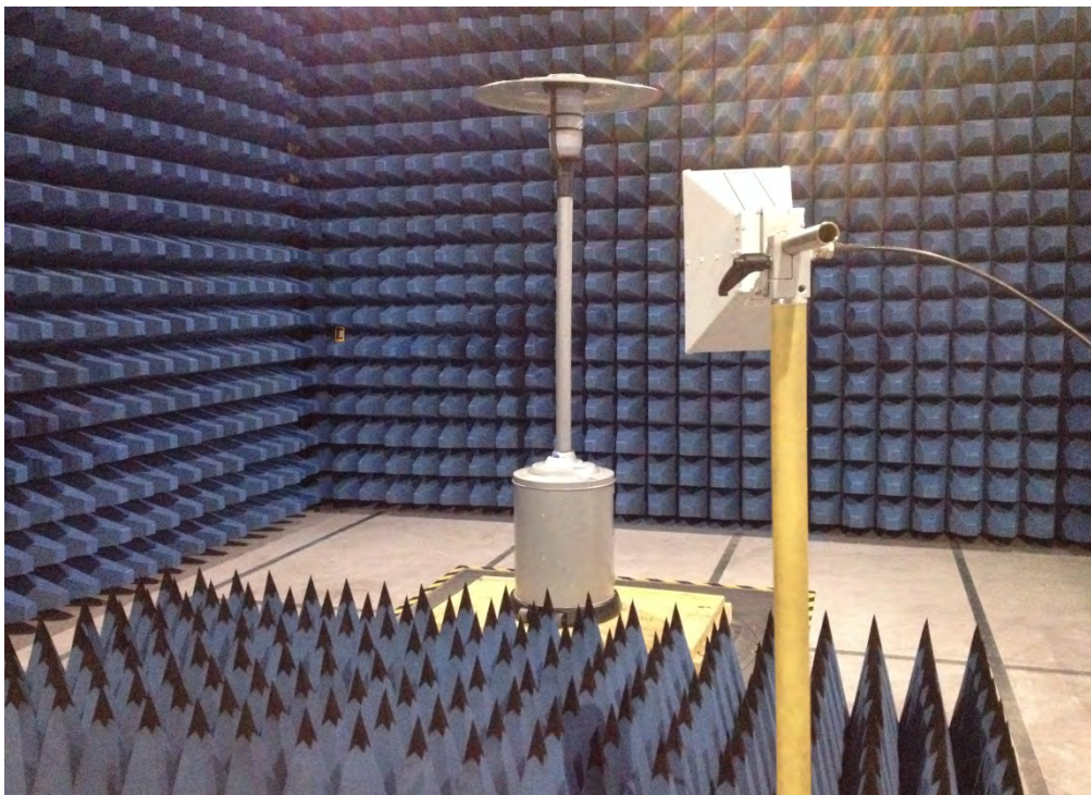
Above 1GHz
