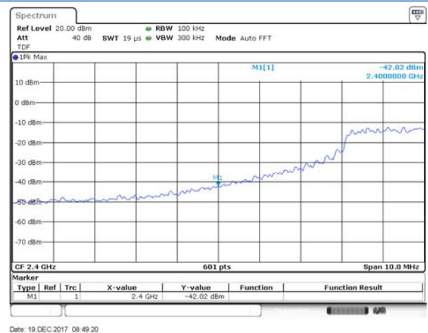
802.11n-20 MHz LOW CHANNEL, Band Edge
