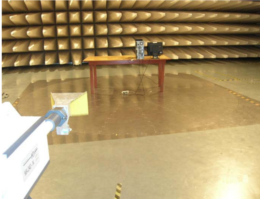
Radiation Test Setup Pictures (High Frequency)
