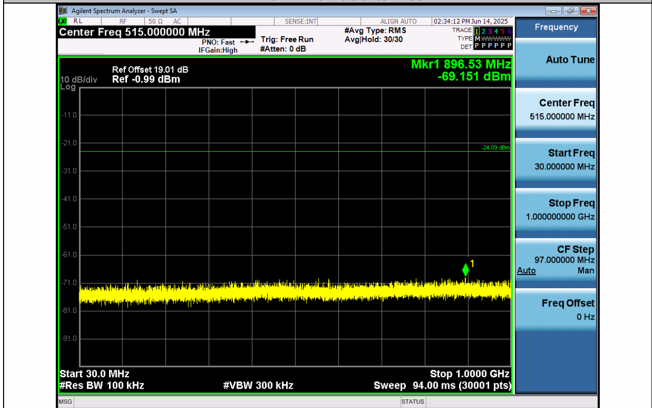
11B-Ant1-2412-30~1000-PASS
