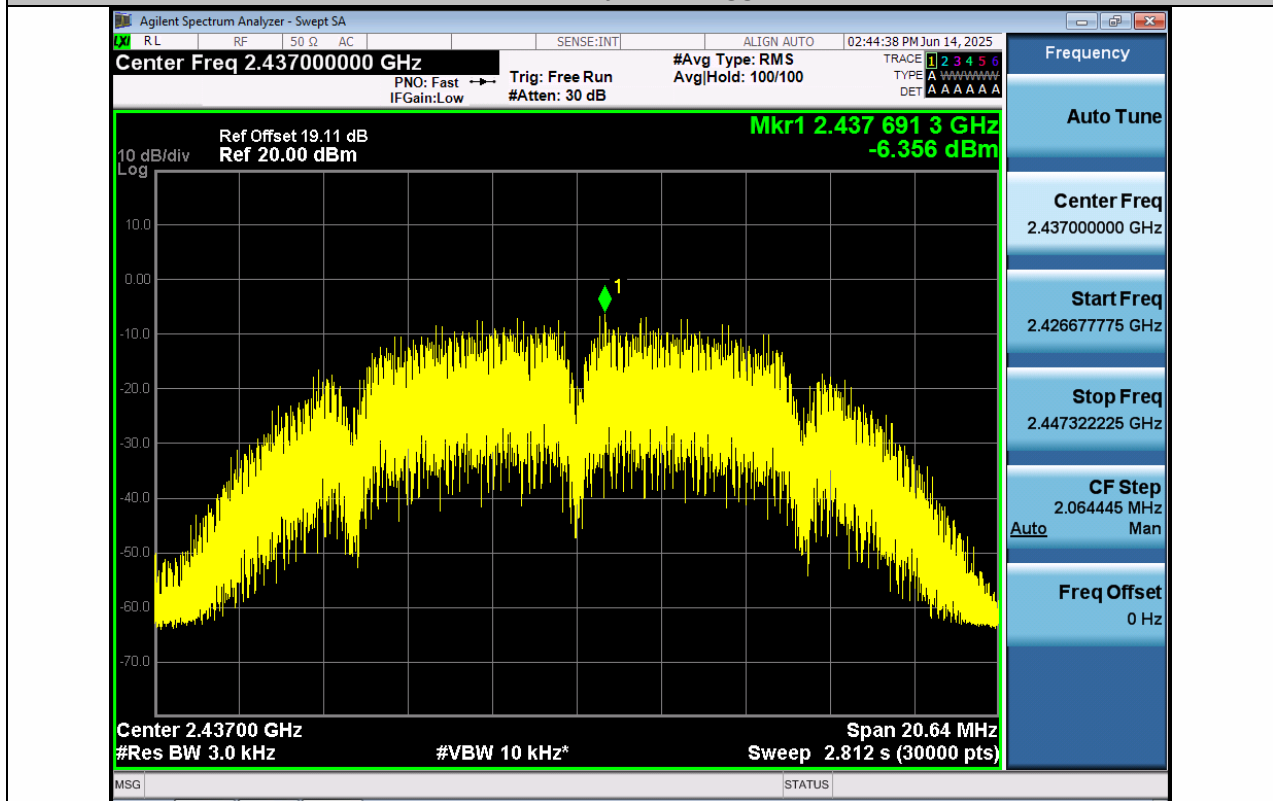
11B-Ant1-2437-PASS
