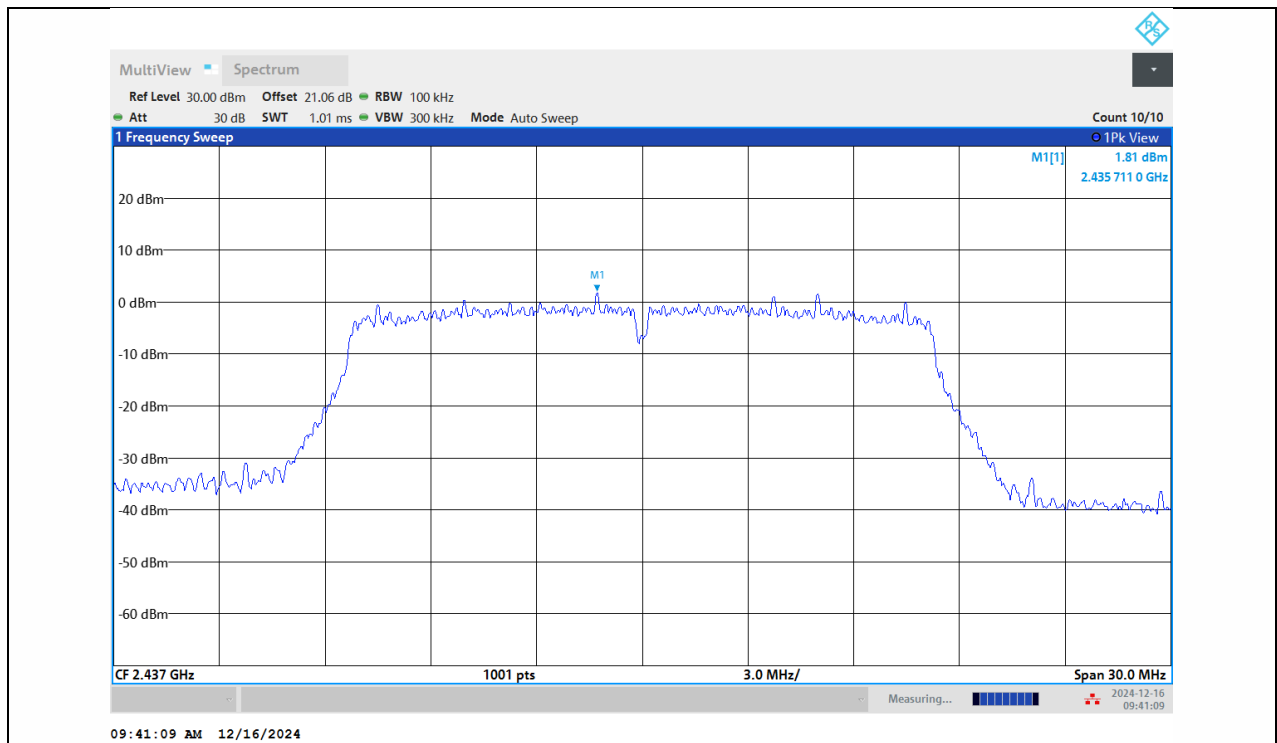
11G-Ant1-2437-0~Reference-PASS
