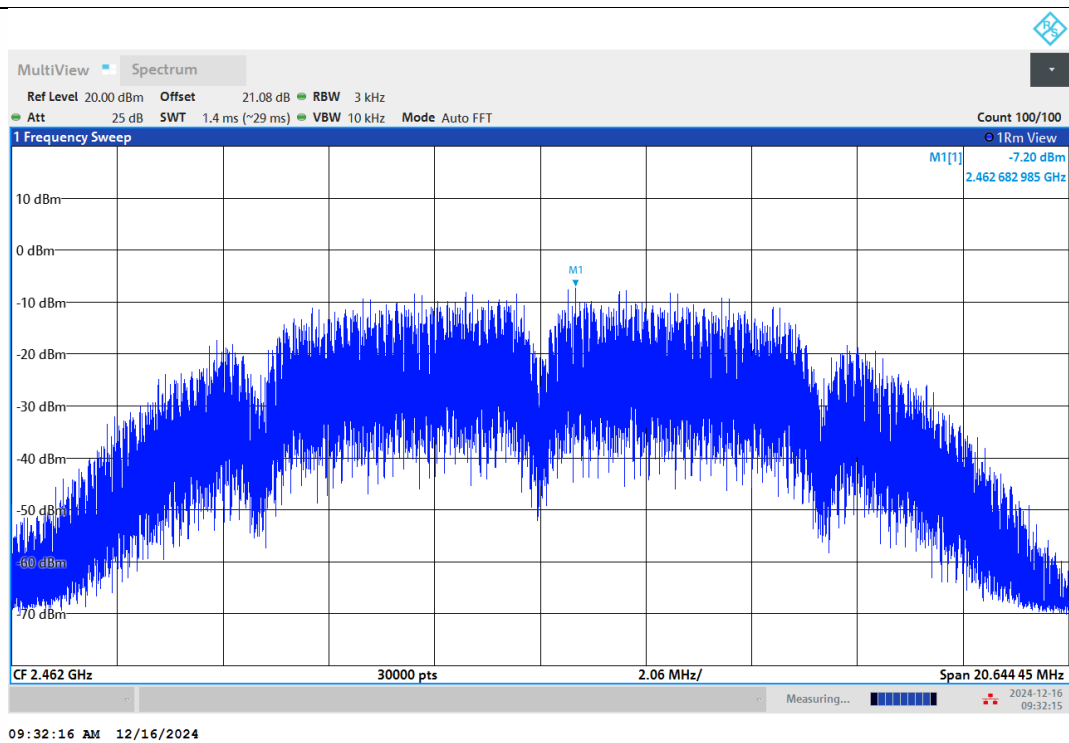
11B-Ant1-2462-PASS
