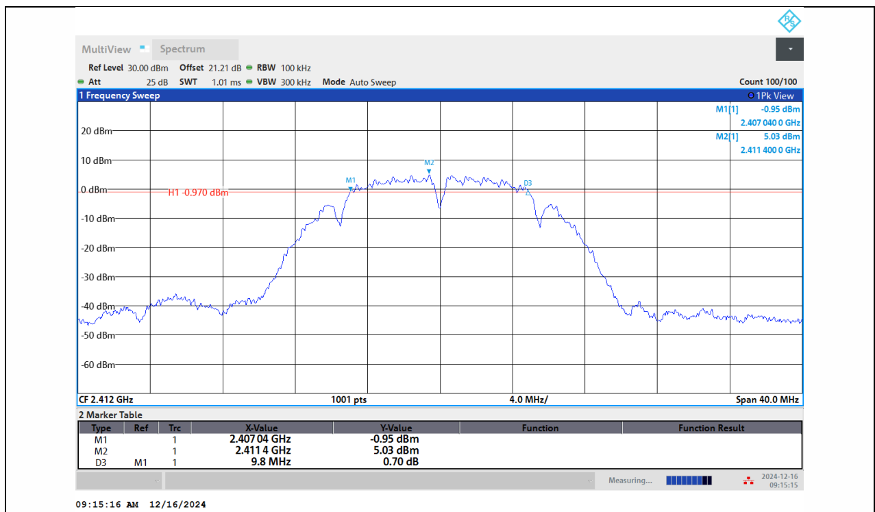
11B-Ant1-2412-PASS
