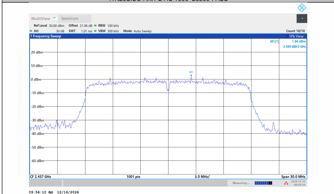
11N20SISO-Ant1-2437-0~Reference-PASS
