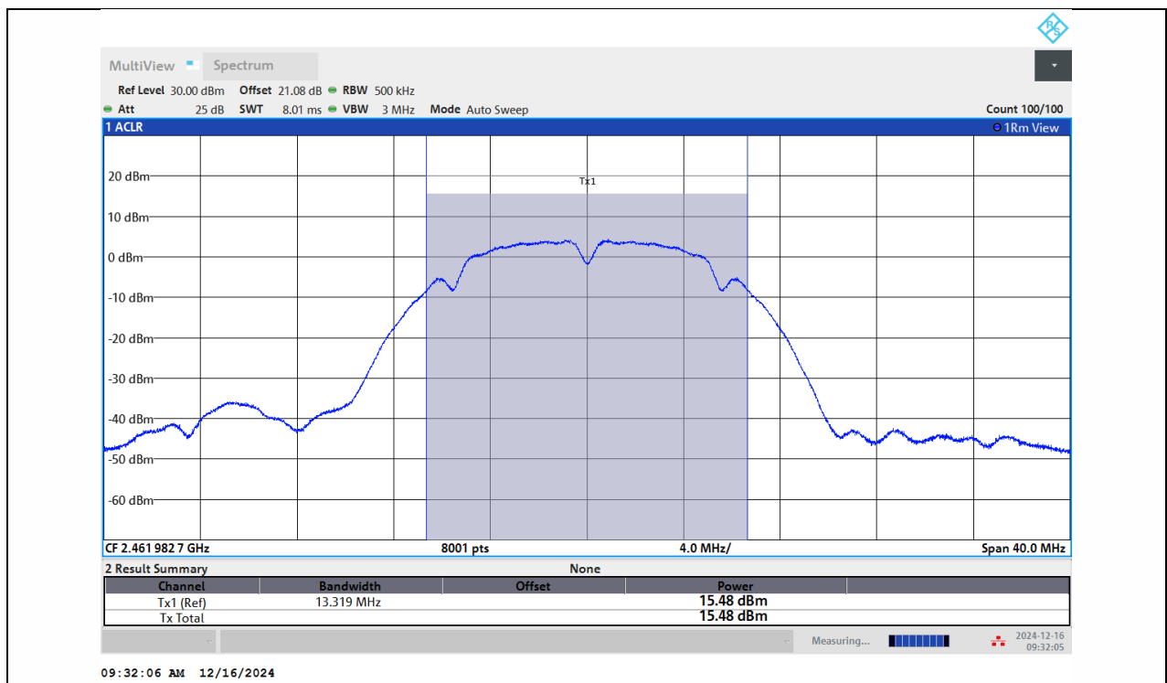
11B-Ant1-2462-PASS
