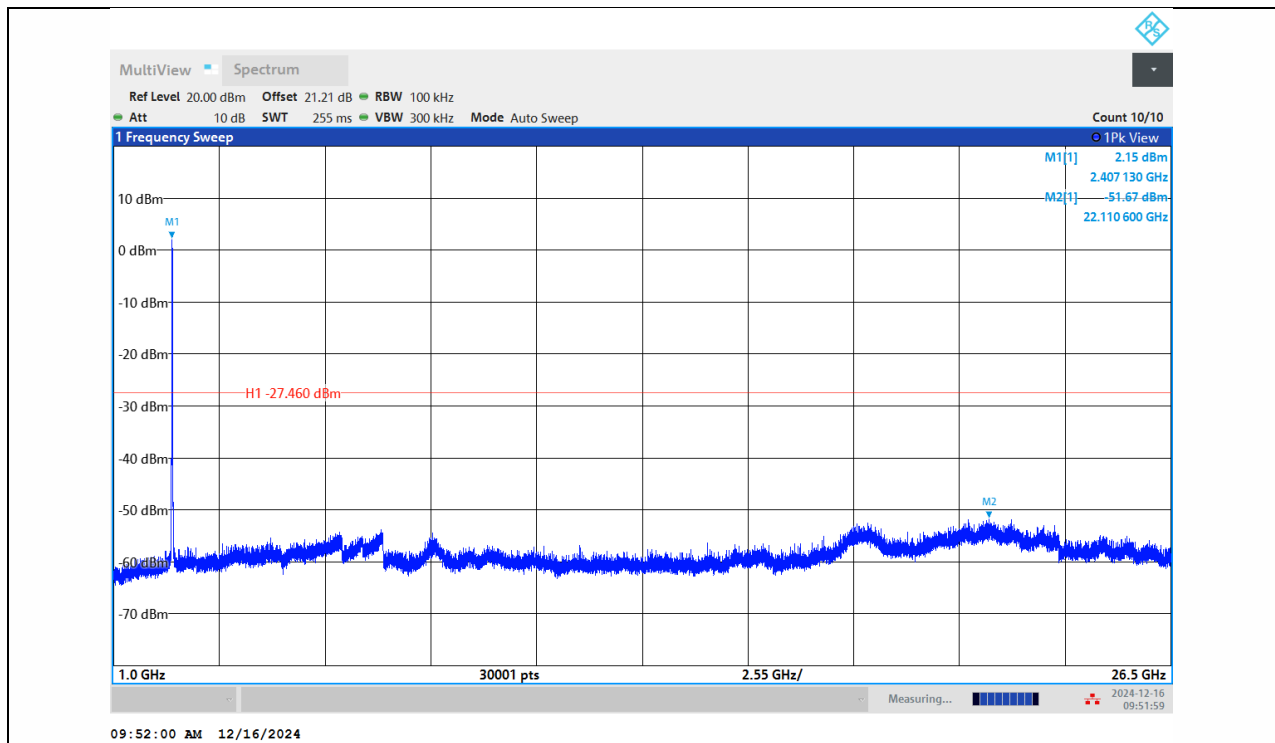
11N20SISO-Ant1-2412-1000~26500-PASS
