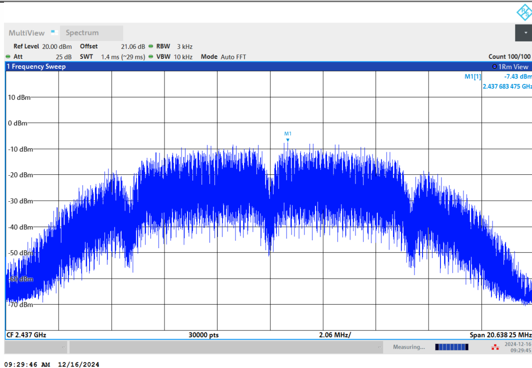
11B-Ant1-2437-PASS
