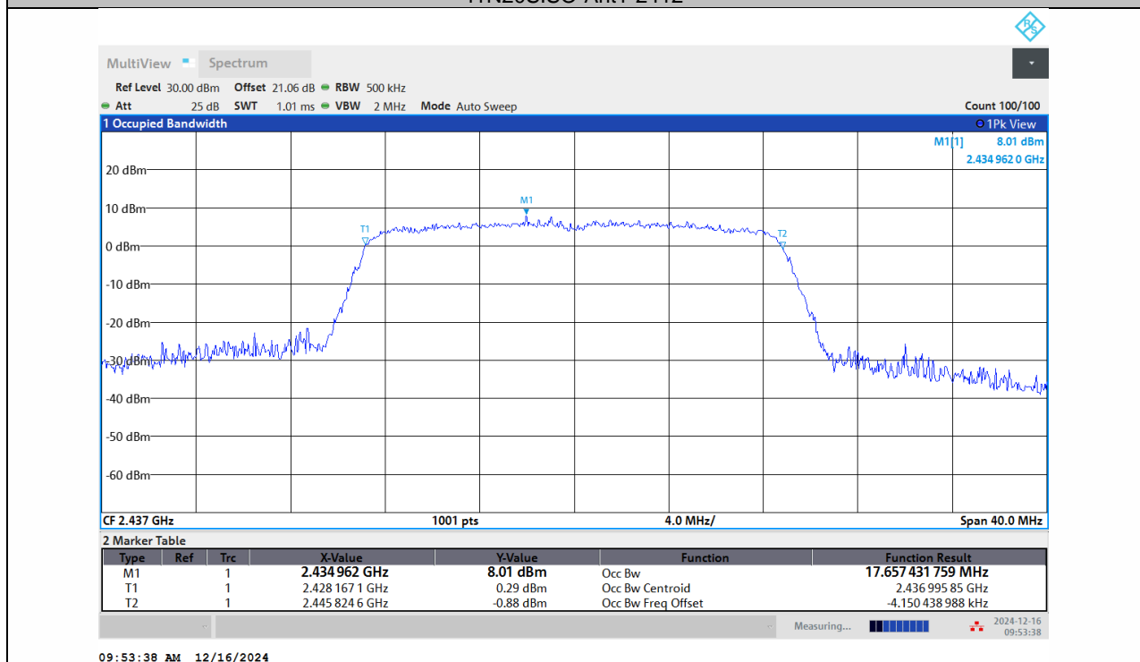
11N20SISO-Ant1-2437
