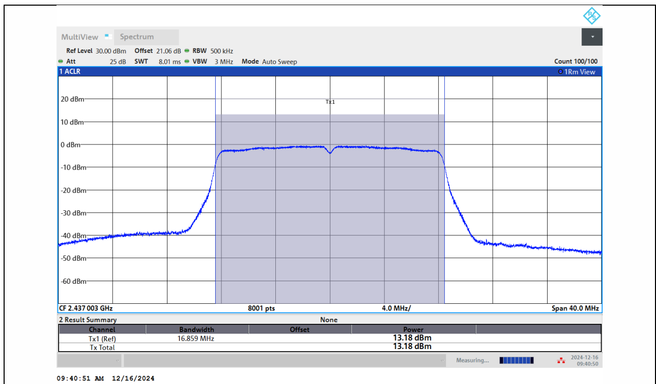
11G-Ant1-2437-PASS
