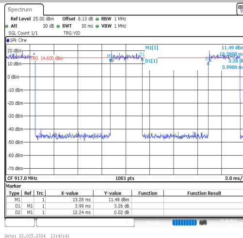
WiFi HaLow (2Mbps)-Ant1-917
