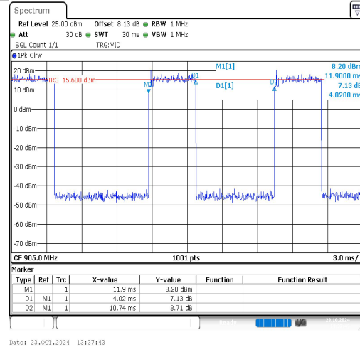
WiFi HaLow (2Mbps)-Ant1-905
