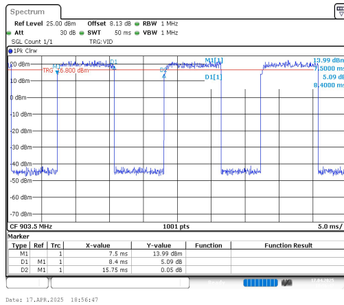
WiFi HaLow (1Mbps)-Ant1-903.5
