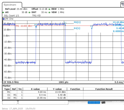
WiFi HaLow (1Mbps)-Ant1-926.5
