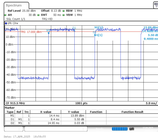
WiFi HaLow (1Mbps)-Ant1-915.5
