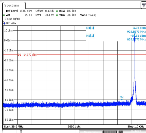
WiFi HaLow (4Mbps)-Ant1-918-30~1000-PASS
