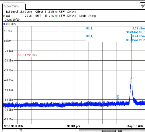
WiFi HaLow (4Mbps)-Ant1-906-30~1000-PASS
