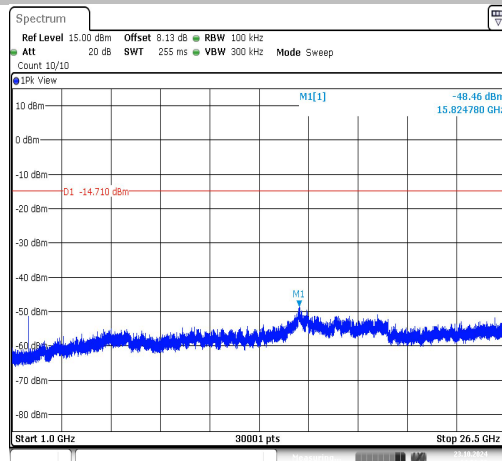
WiFi HaLow (4Mbps)-Ant1-906-1000~26500-PASS
