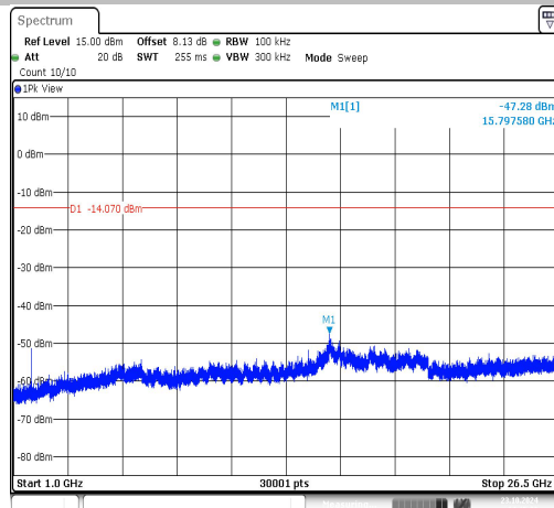
WiFi HaLow (4Mbps)-Ant1-918-1000~26500-PASS
