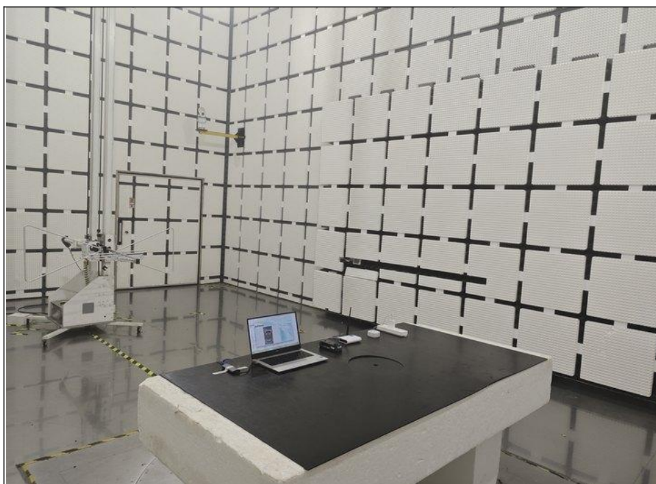
RADIATED EMISSION TEST (Below 1GHz)
