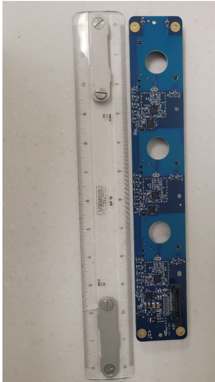
NGI PCB side 1
