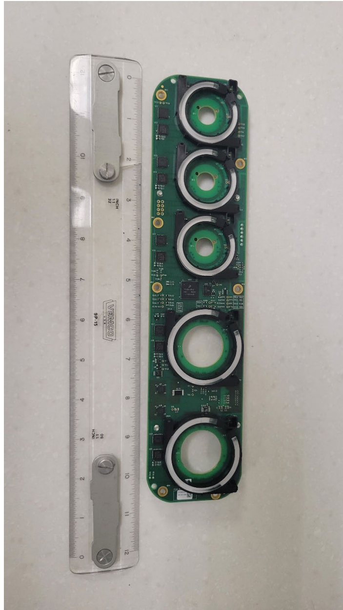
Pneumatic PCB side 1
