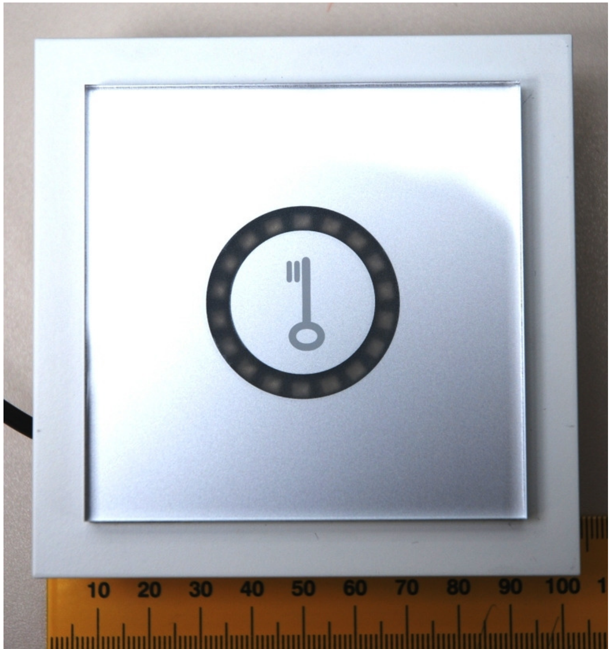
Fig. 3 Front side – Models 860 and 861 with front plastic cover
