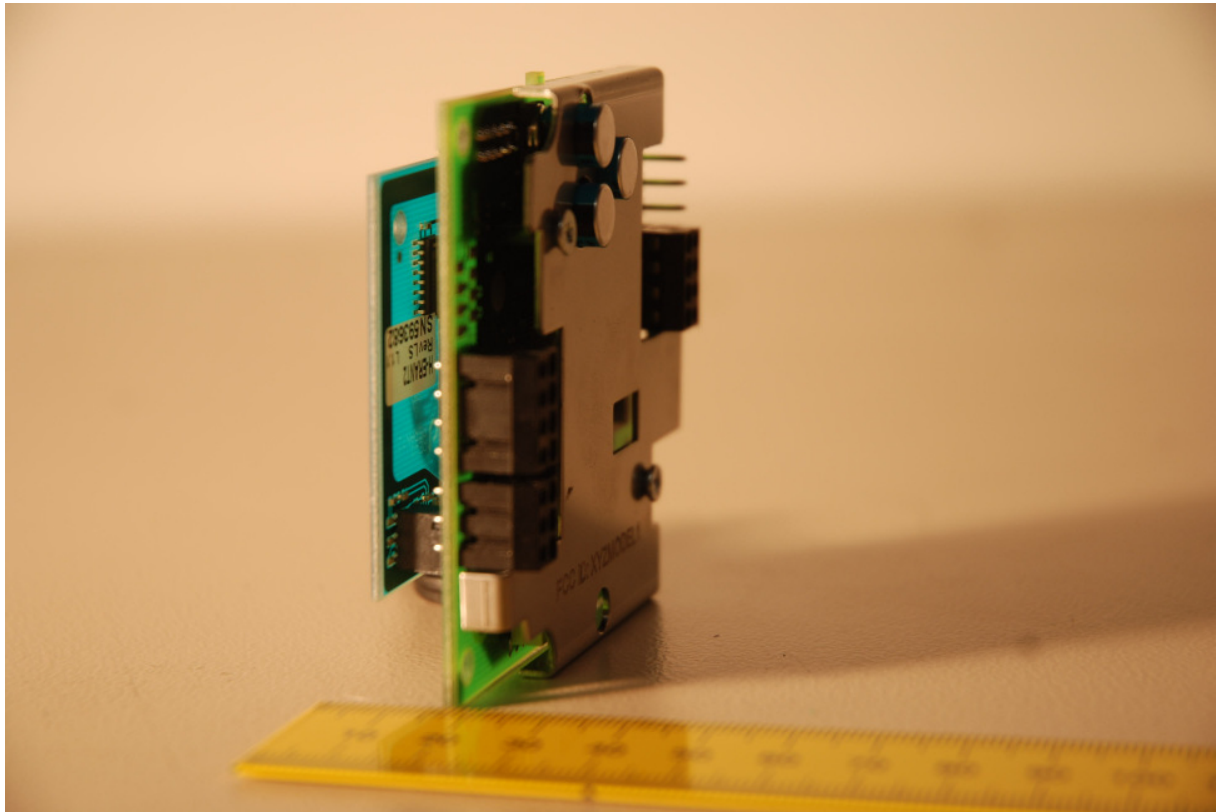
Fig. 3 ERT 661 Side view
