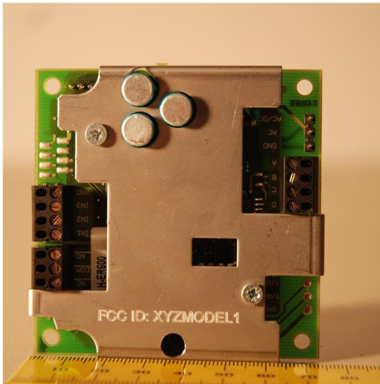
Fig. 2 ERT 660 and ERT 661 with shielding - Rear view with FCC label
