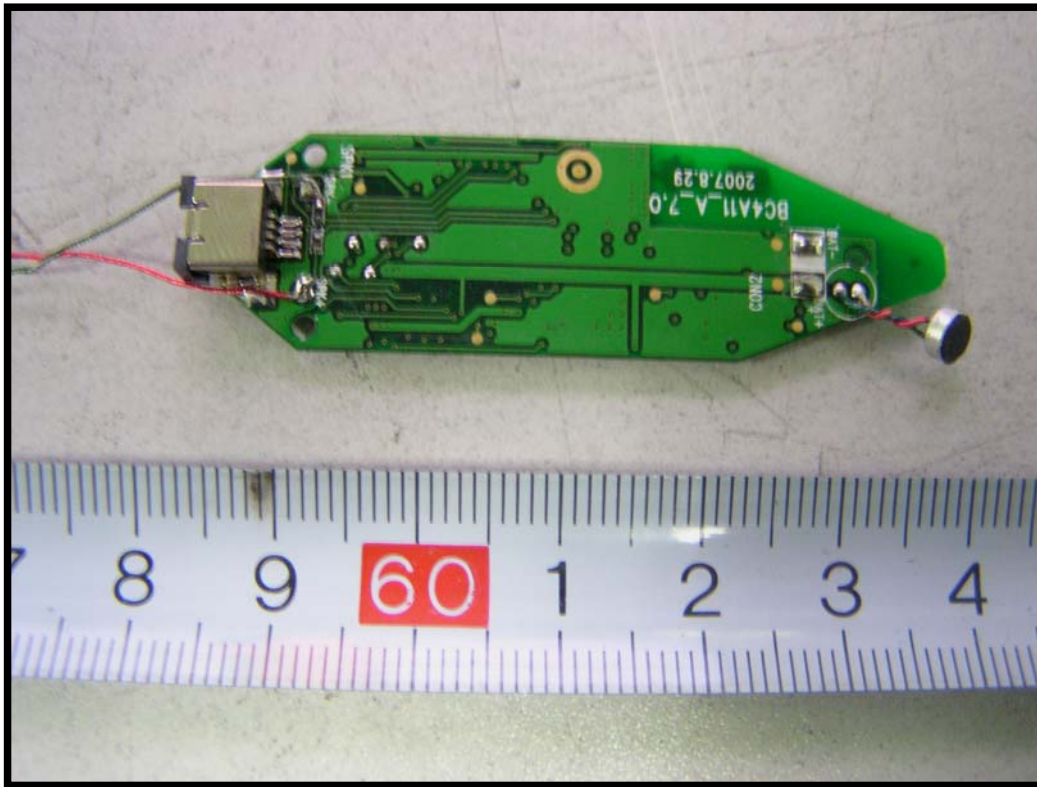
Main Board Bottom Components View
