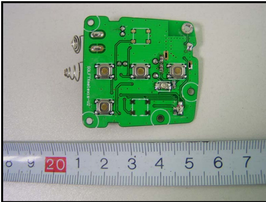
EUT- Main Board Components Bottom View
