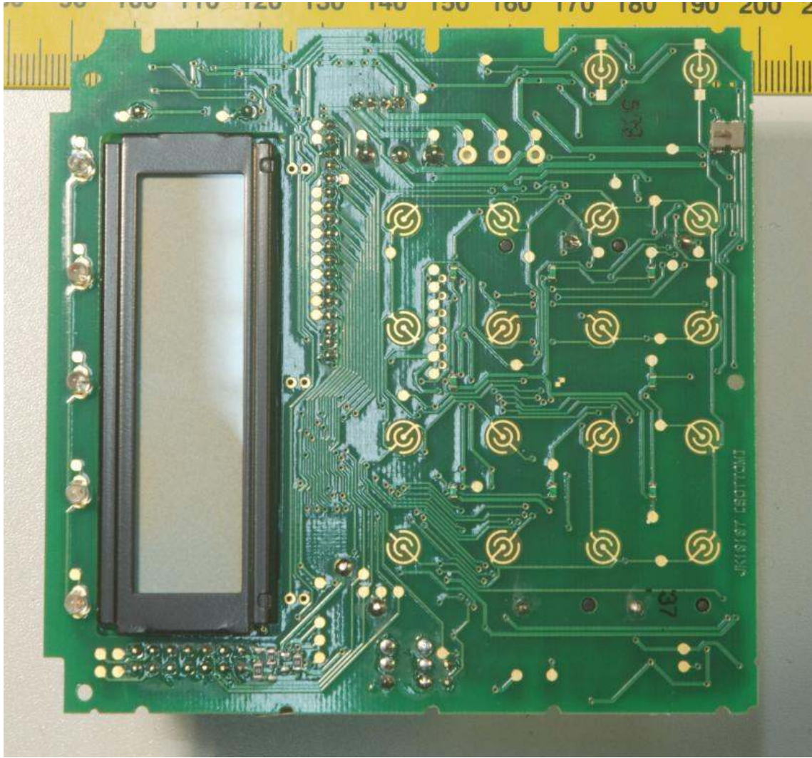
PCB view keyboard side
