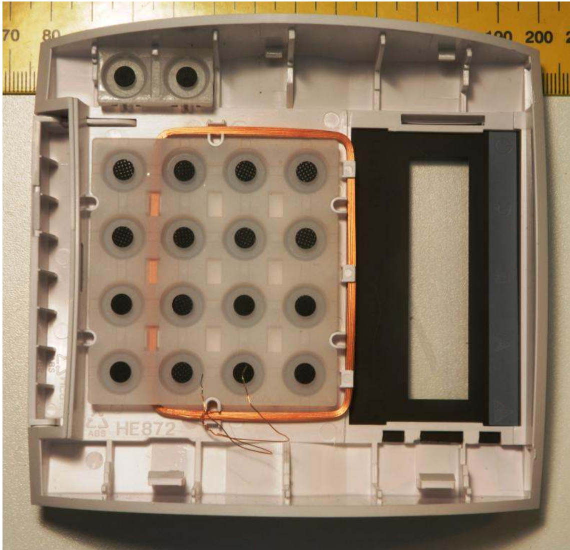
Keyboard from inside with card reader antenna
