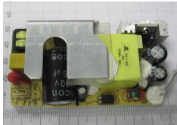
PCB side 1,
