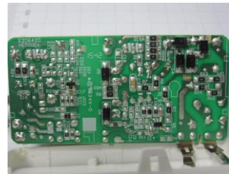
PCB side 2
