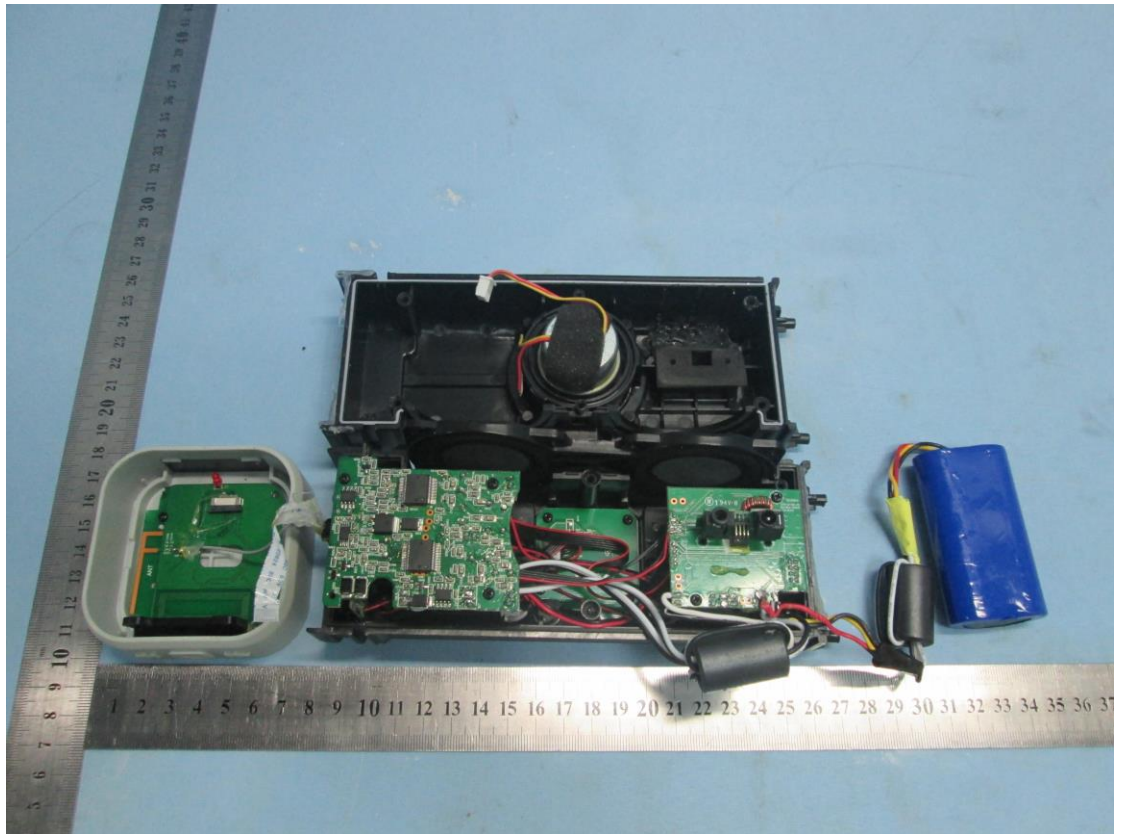
Internal photos of EUT:
