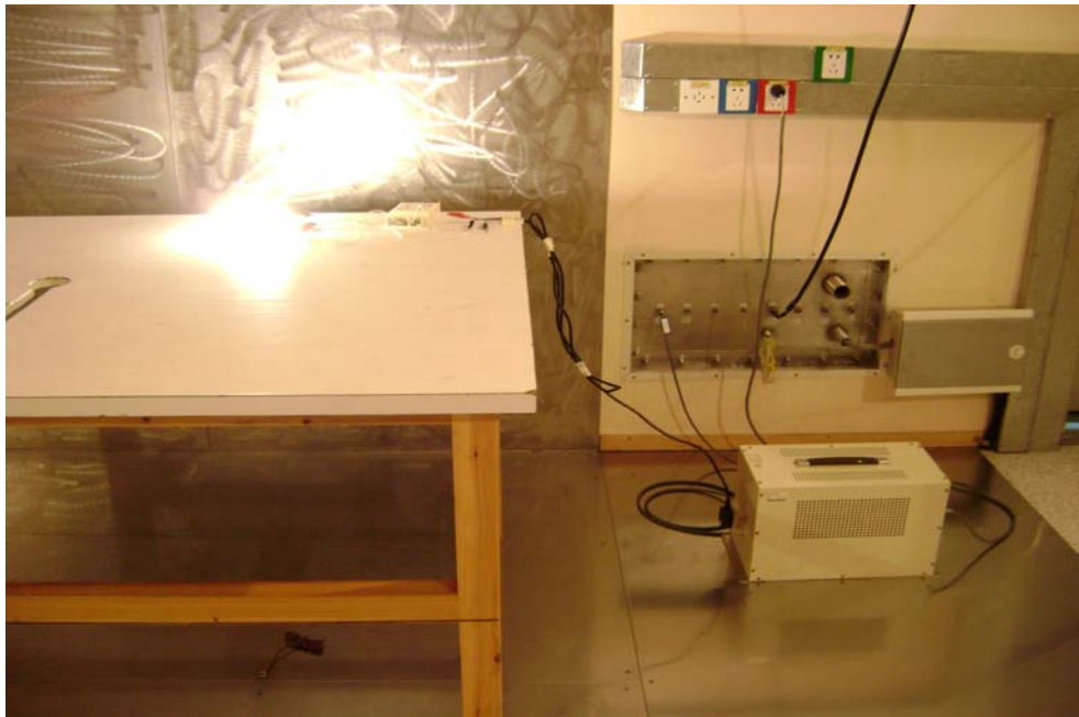
Conducted Emission Test View for LEB-214~218
