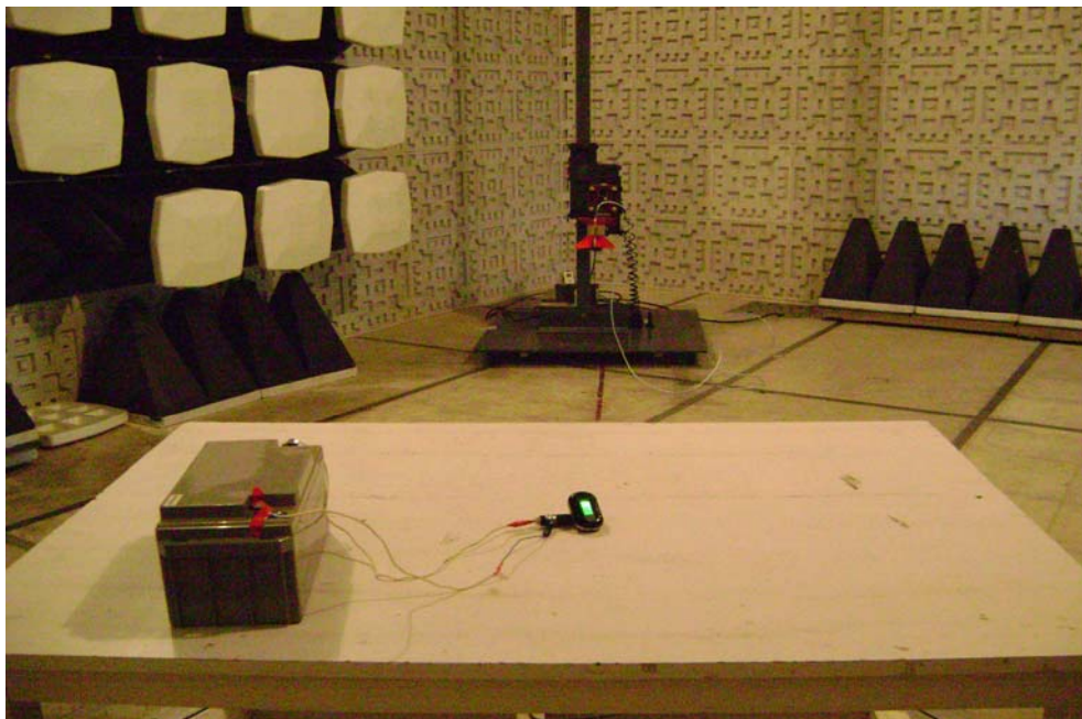
Bluetooth Part Radiation Emission Test View For 1GHz-25GHz
