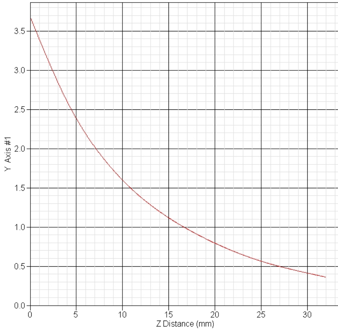
SAR-Z Axis at Hotspot x:10.20 y:1.80
