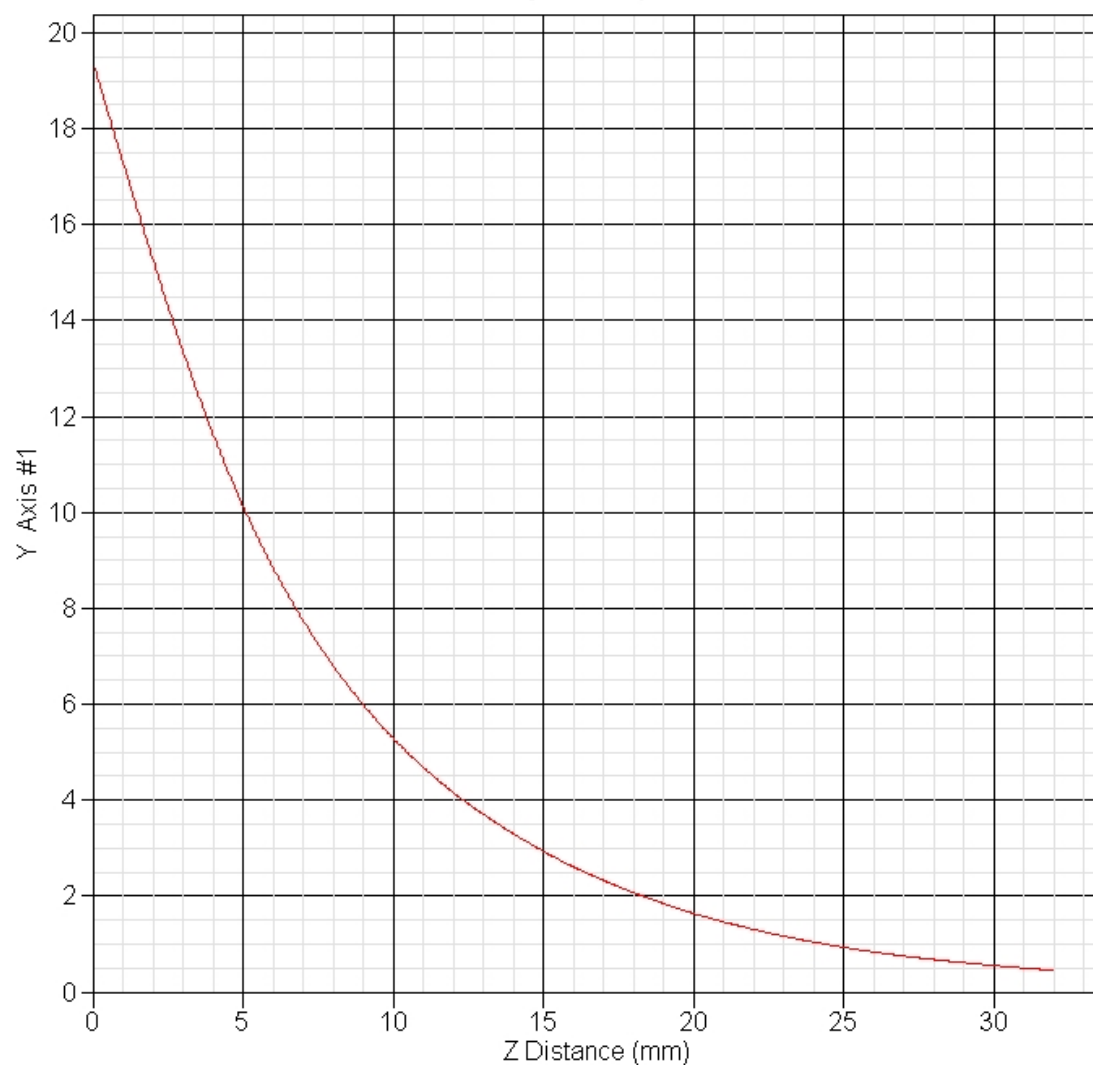
SAR-Z Axis at Hotspot x:10.30 y:-2.00
