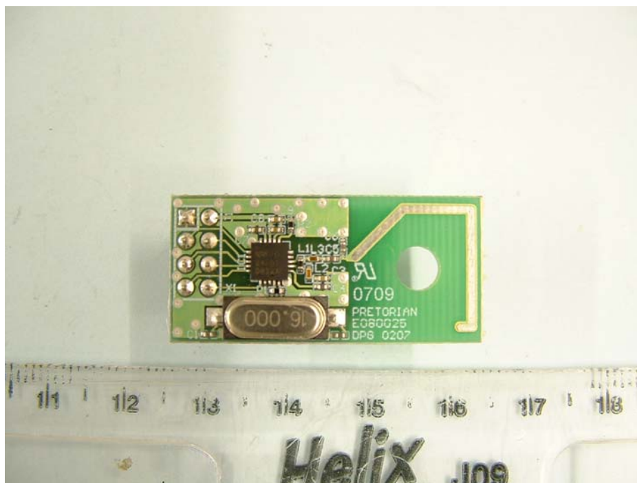
Radio Module Component Side
