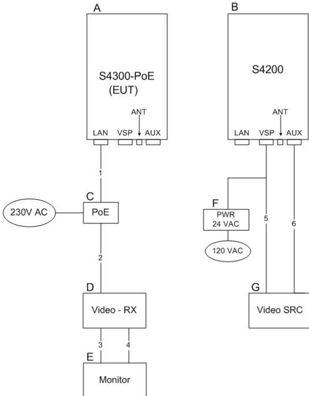
Figure 3. Block Diagram of Test Configuration (S4300)
