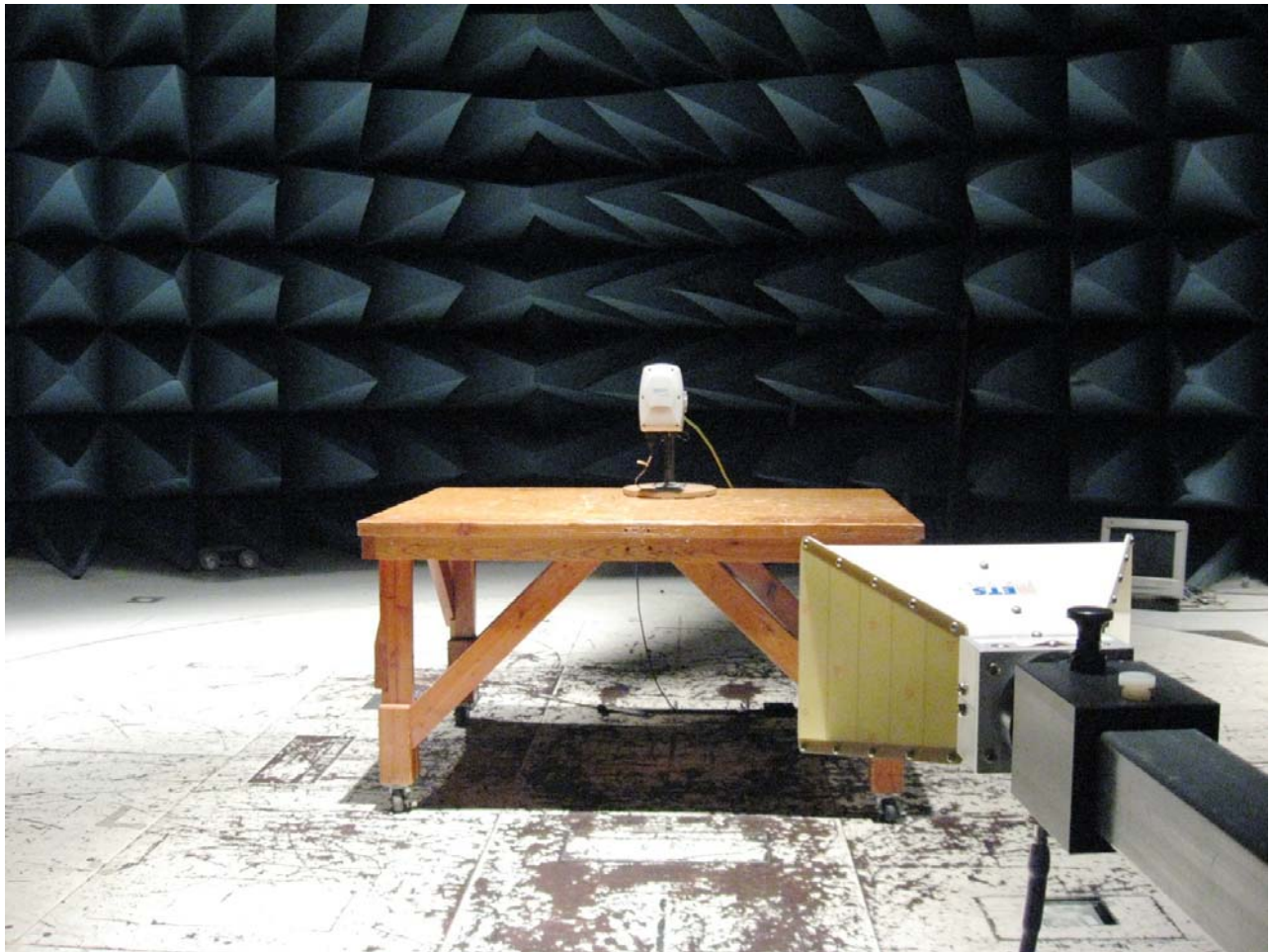
Photograph 4. Radiated Emission Limits Test Setup 1 - 5GHz
