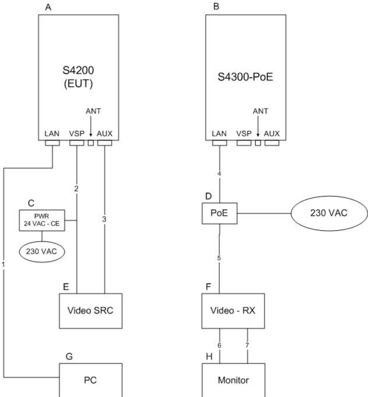
Figure 2. Block Diagram of Test Configuration (S4200)
