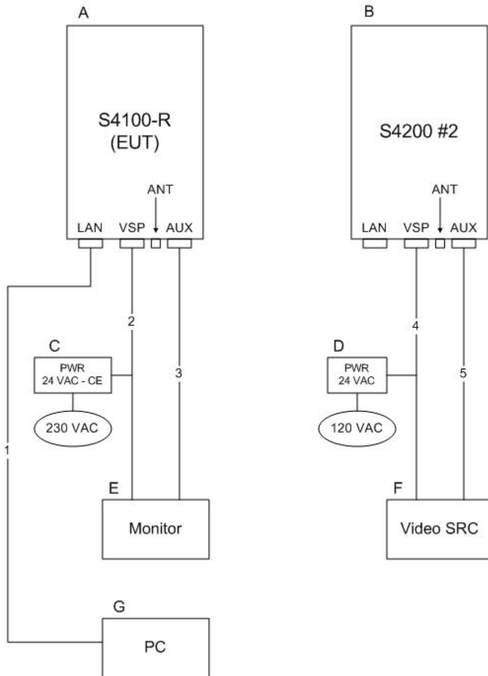
Figure 1. Block Diagram of Test Configuration (S4100)
