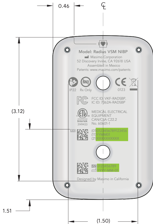
Location Requirement (1:1 scale in inches) Tolerance: +/- 0.015"
