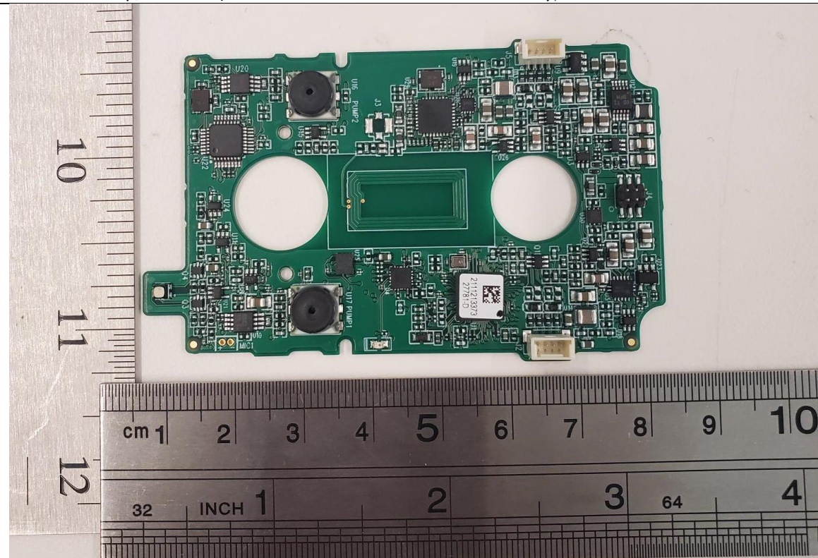
Front view of p/n: 27781(Griffon NiBP V3 Circuit Board Assembly) without foam
