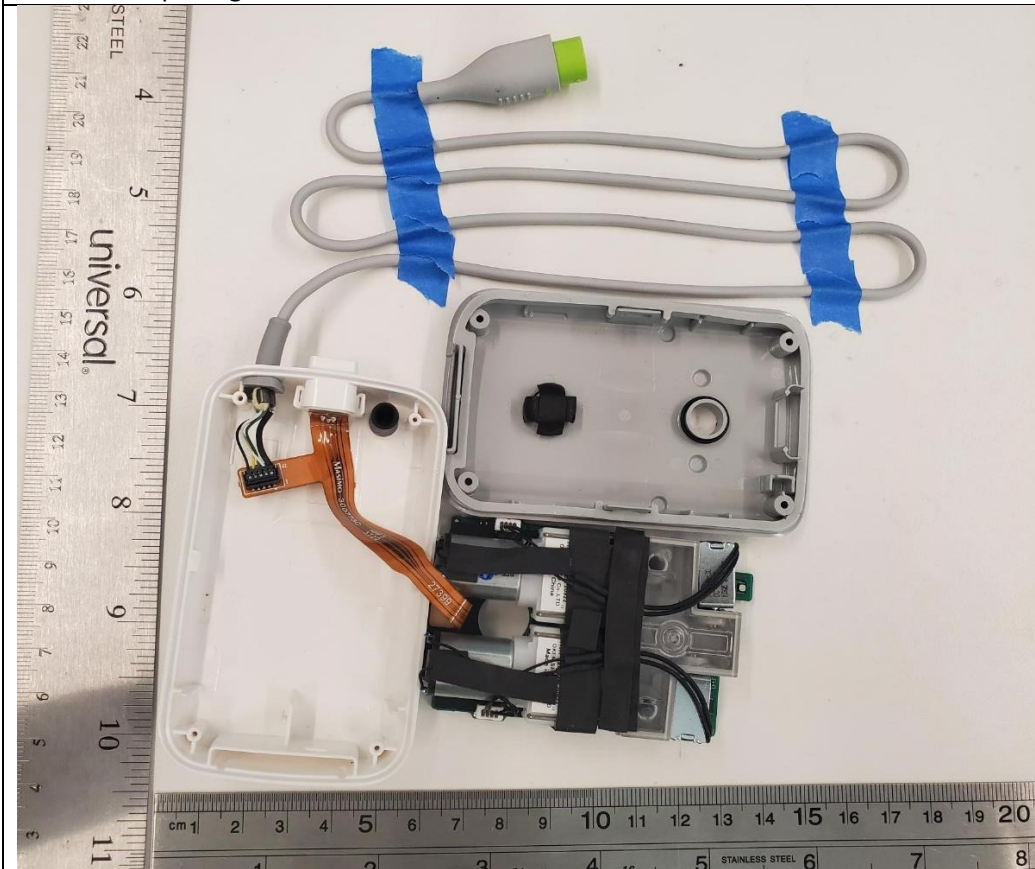
View after opening back cover showing other side of the 27781
