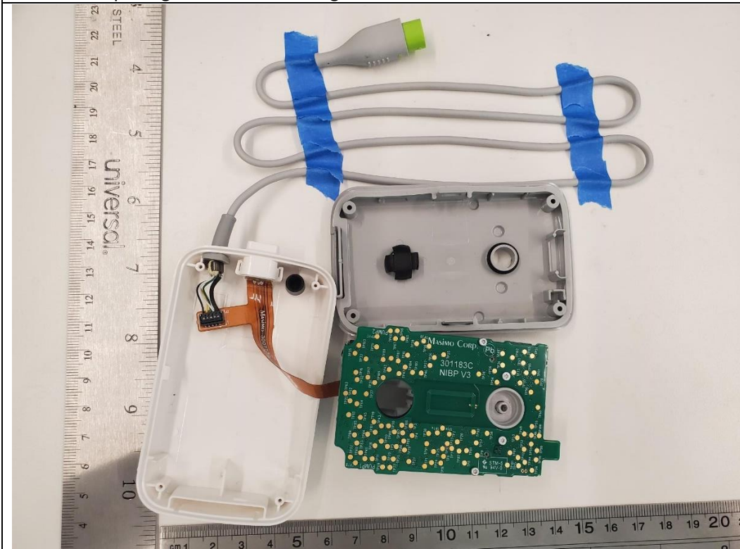
View after opening back cover showing other side of the 27781
