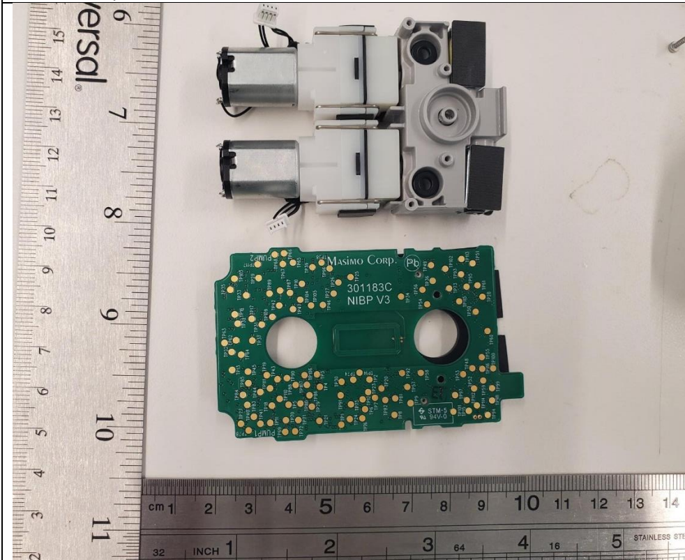
Back view of p/n: 27781 (Griffon NiBP V3 Circuit Board Assembly) with assembly, Wire Harness, Griffon Pump + Valve
