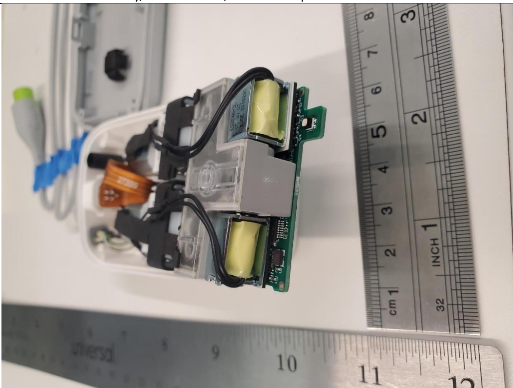
Closer view of assembly, Wire Harness, Griffon Pump + Valve
