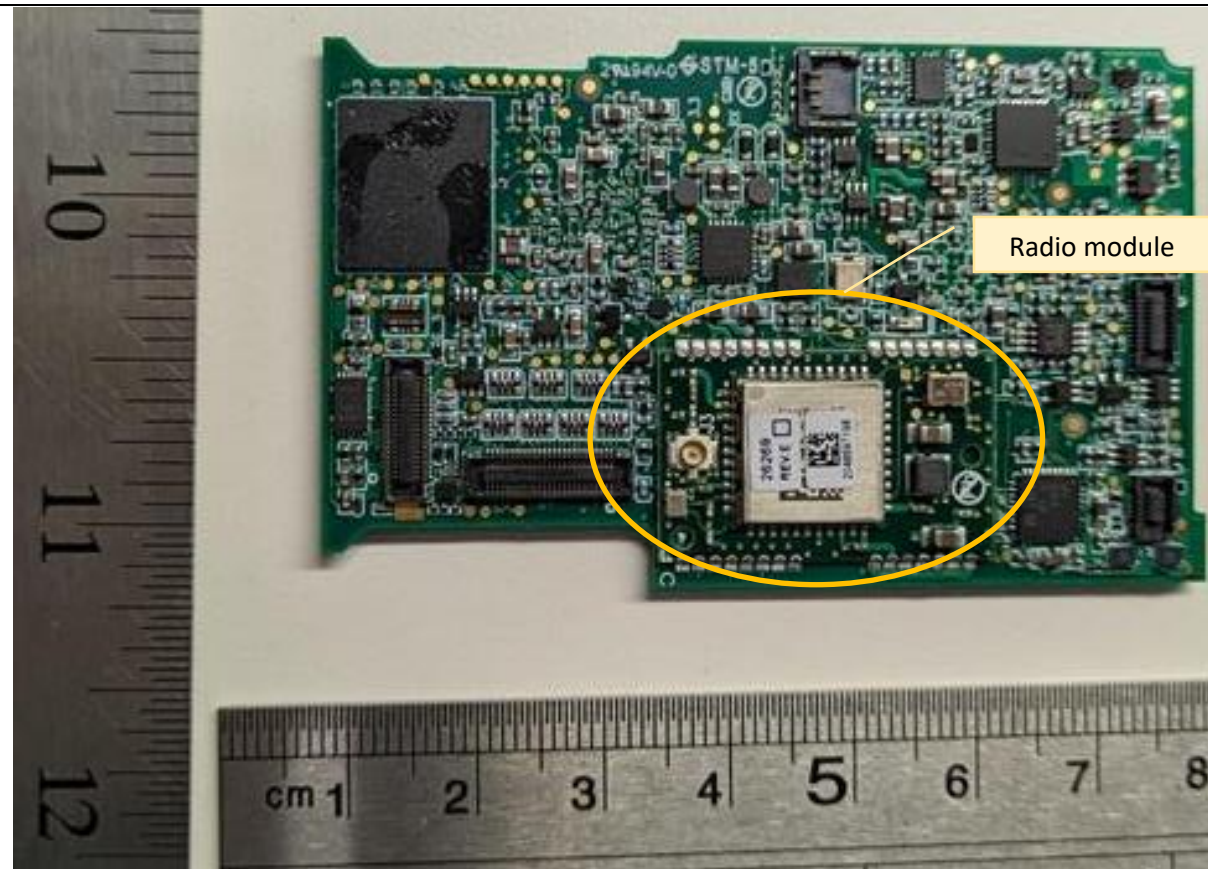
PCB back
