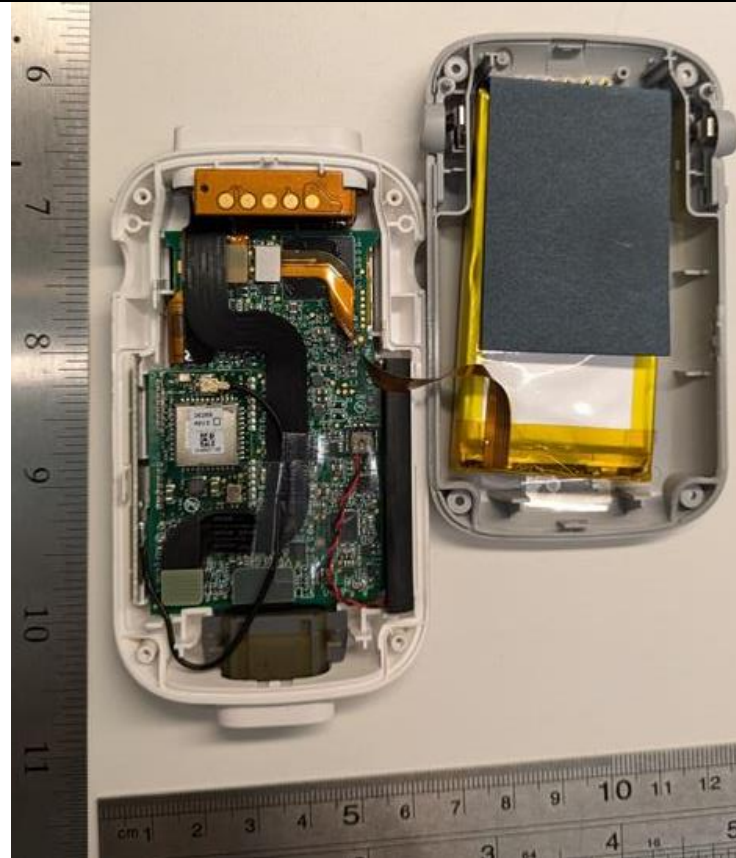
Battery removed
