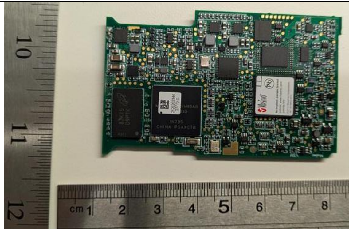
PCB front
