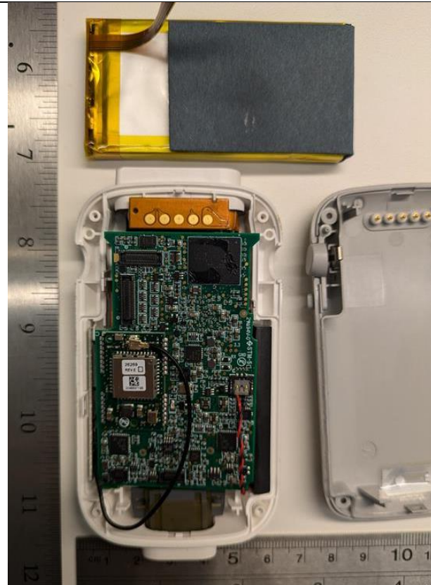
Battery removed
