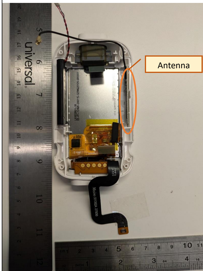
Top enclosure cover without PCB-2 providing flex details
