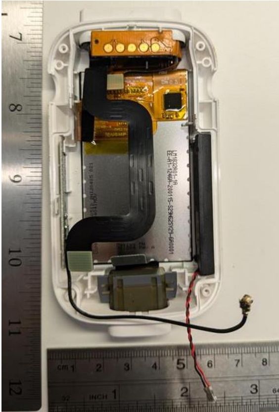
Top enclosure cover without PCB-1
