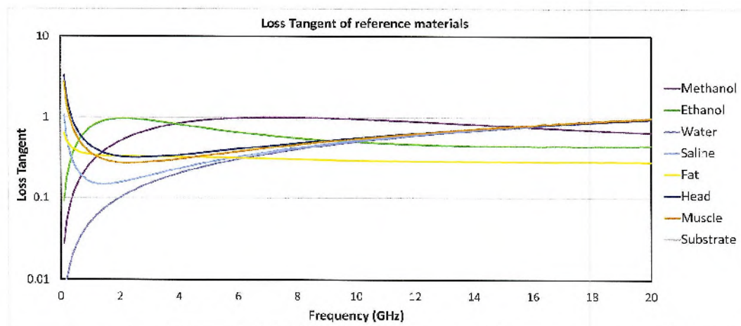
Fig. B.3 Loss tangent of reference materials
