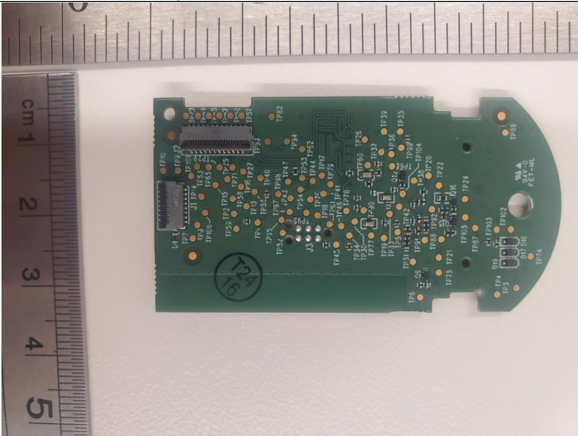
Radio back side Printed Wiring Board
