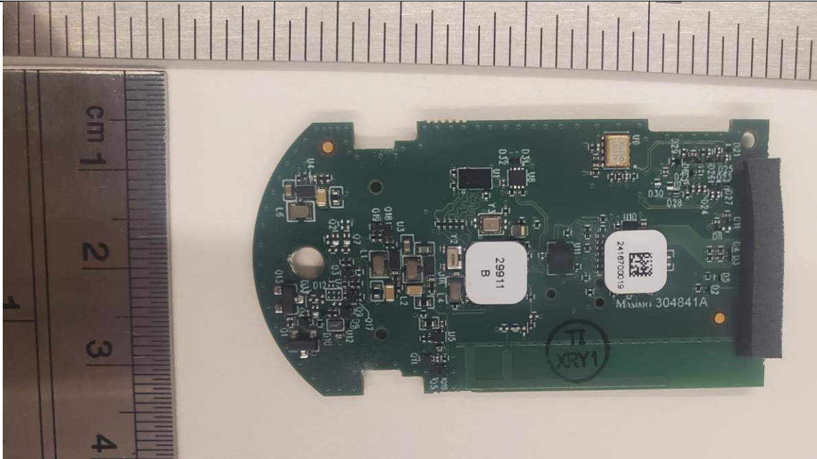
Radio front side Printed Wiring Board
