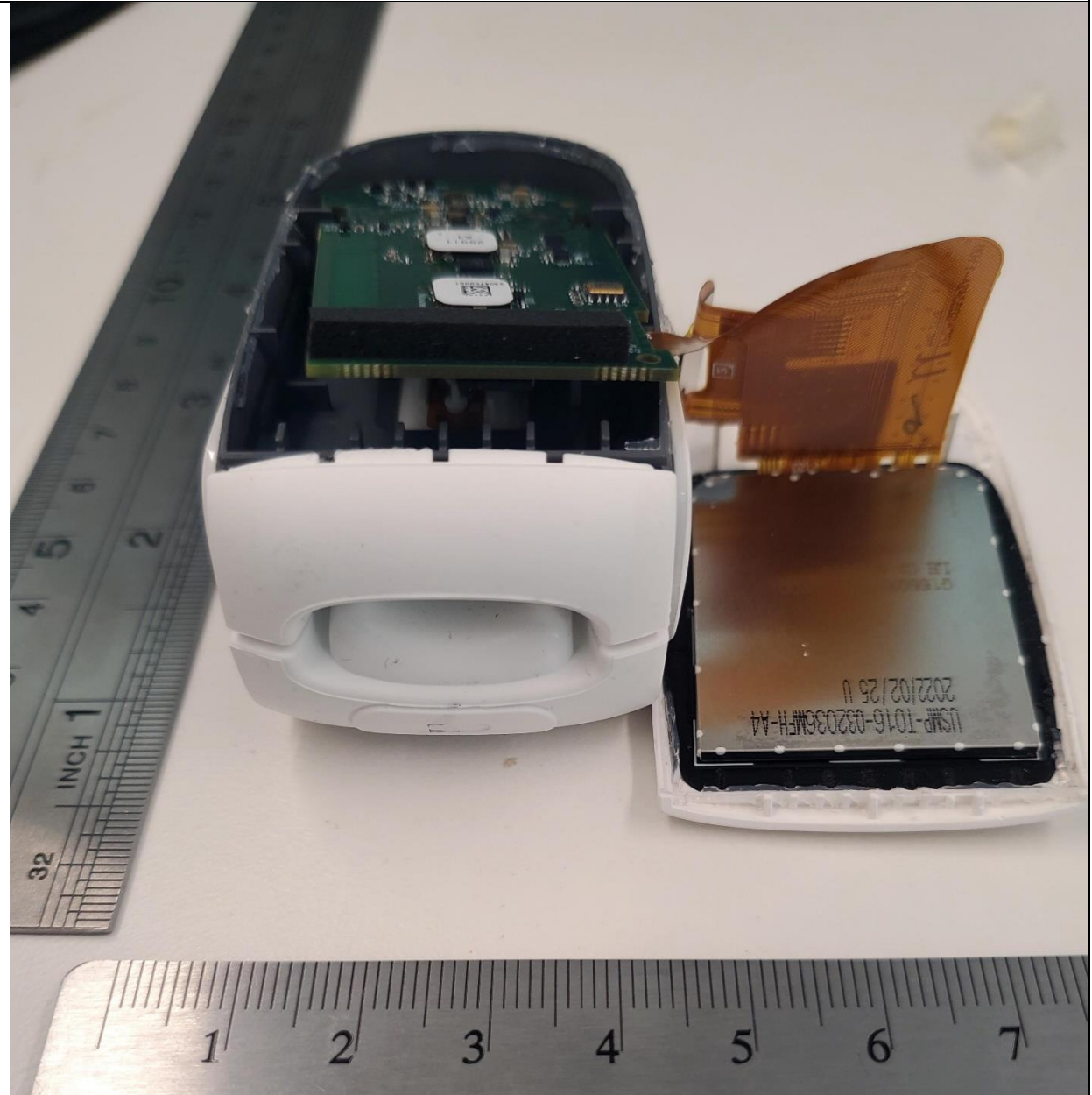
Internal view between the board 29911 and front cover with display to uncover the flex
