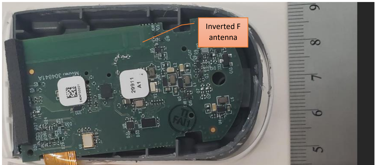
Figure 1: Printed Inverted-F Antenna
