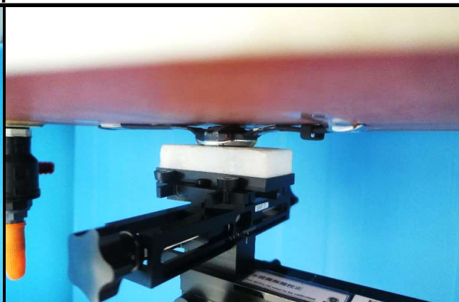
Rear Face of EUT Tested at 0 mm for NFC
