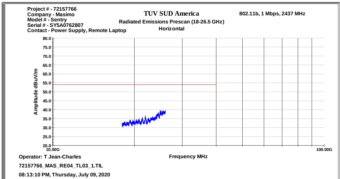
Figure 2.2.7-6: Radiated Emissions Representative Scan 18 GHz – 26 GHz – Horizontal Polarization – Wi-Fi
