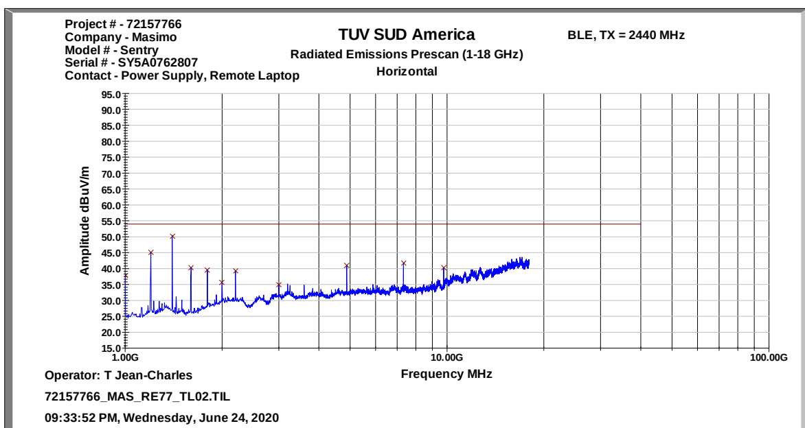
Figure 2.2.7-11: Radiated Emissions Representative Scan 1 GHz – 18 GHz – Horizontal Polarization – BLE
