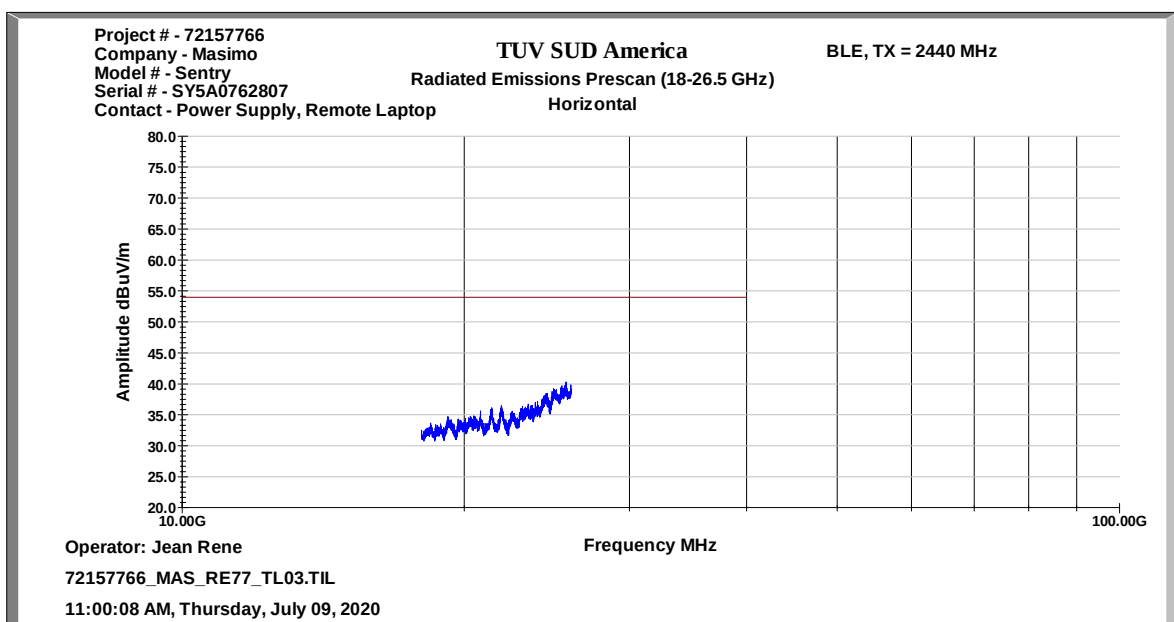
Figure 2.2.7-13: Radiated Emissions Representative Scan 18 GHz – 26 GHz – Horizontal Polarization – BLE
