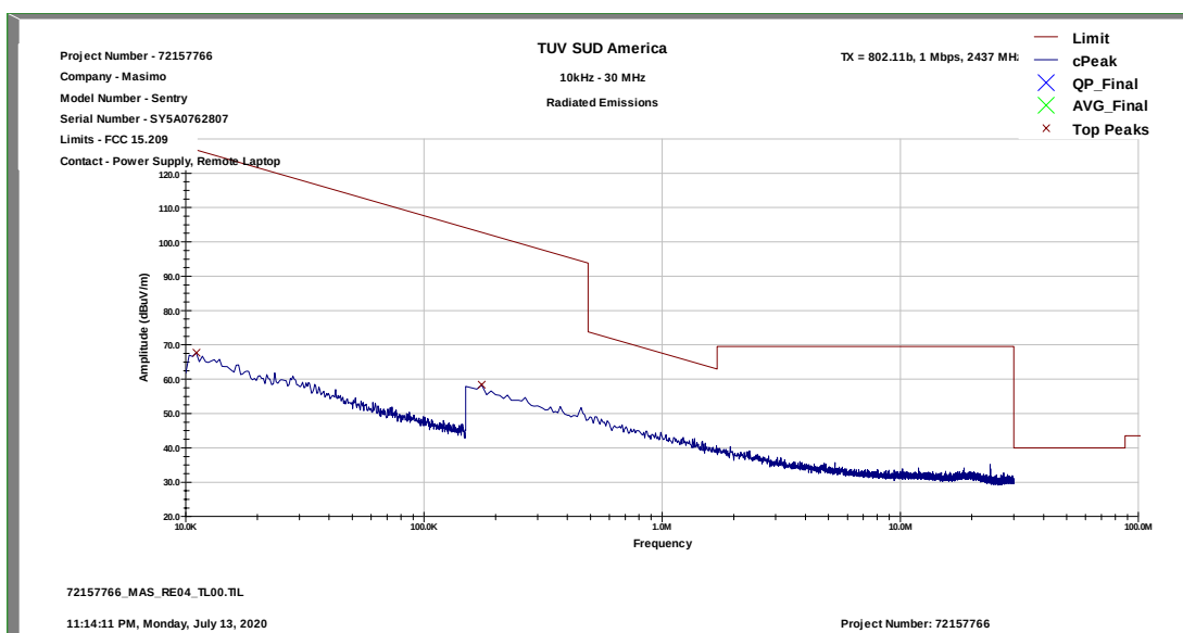
Figure 2.2.7-1: Radiated Emissions Representative Scan below 30 MHz – Wi-Fi
