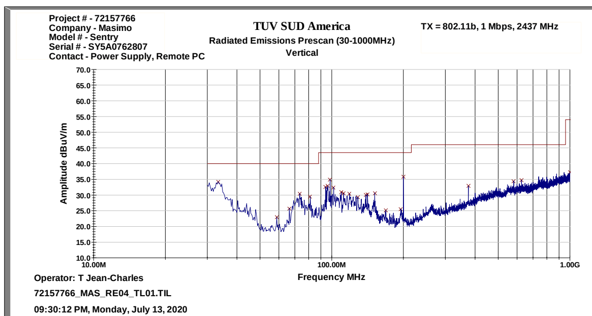
Figure 2.2.7-3: Radiated Emissions Representative Scan 30 MHz – 1 GHz – Vertical Polarization – Wi-Fi
