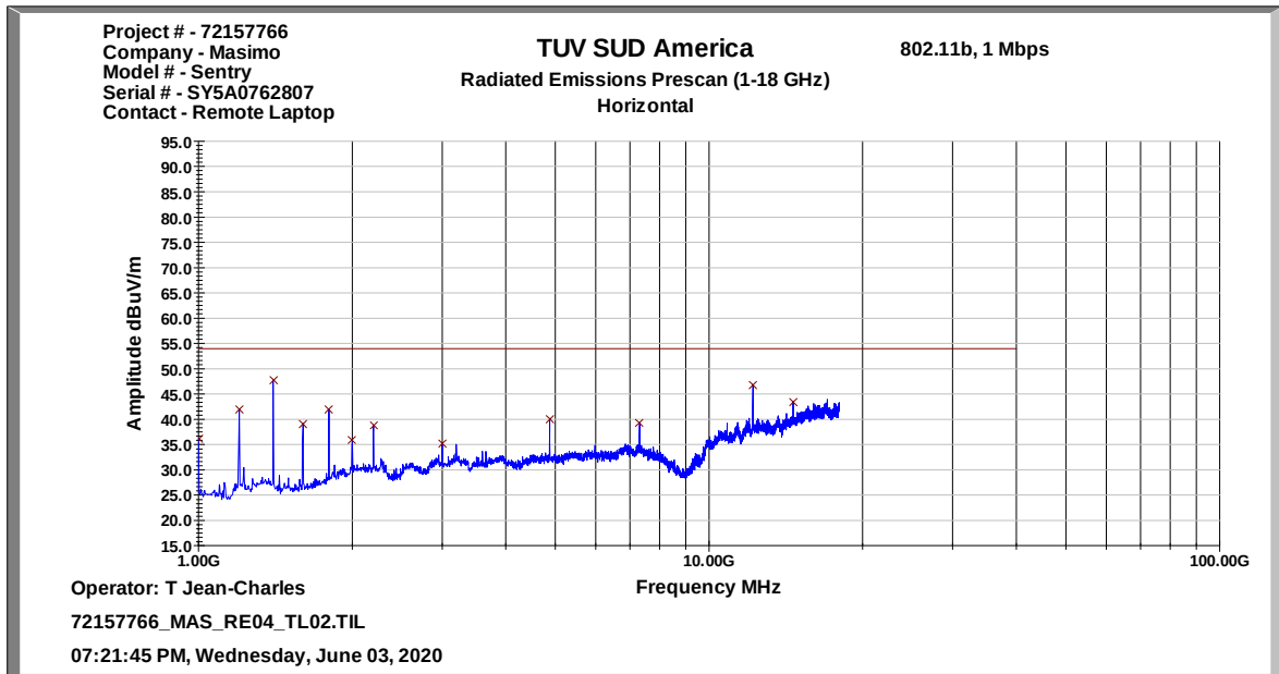
Figure 2.2.7-4: Radiated Emissions Representative Scan 1 GHz – 18 GHz – Horizontal Polarization – Wi-Fi
