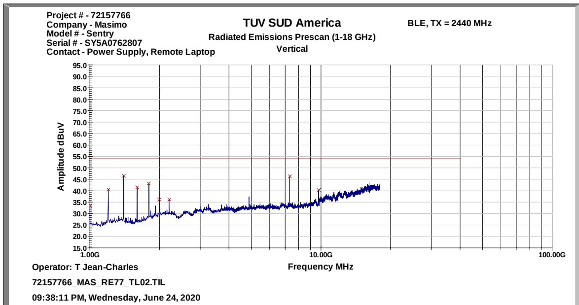
Figure 2.2.7-12: Radiated Emissions Representative Scan 1 GHz – 18 GHz – Vertical Polarization – BLE
