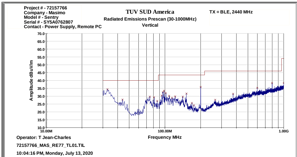
Figure 2.2.7-10: Radiated Emissions Representative Scan 30 MHz – 1 GHz – Vertical Polarization – BLE
