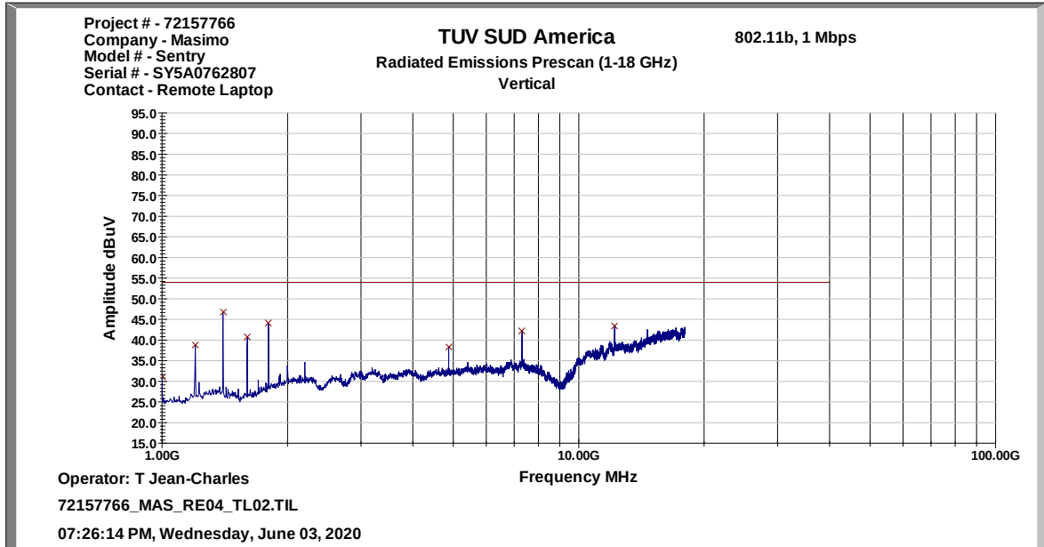
Figure 2.2.7-5: Radiated Emissions Representative Scan 1 GHz – 18 GHz – Vertical Polarization – Wi-Fi
