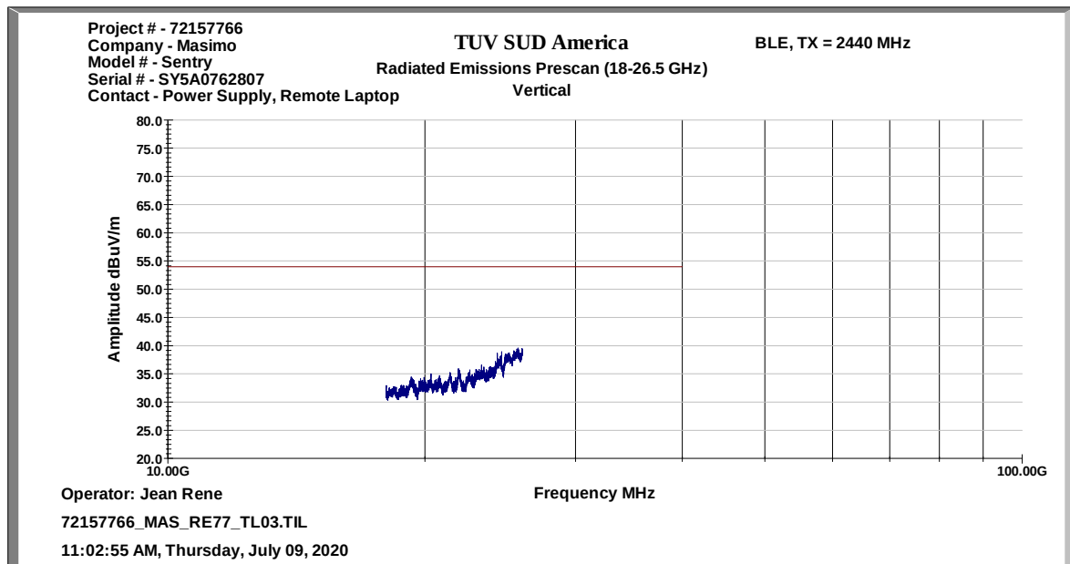
Figure 2.2.7-14: Radiated Emissions Representative Scan 18 GHz – 26 GHz – Vertical Polarization – BLE
