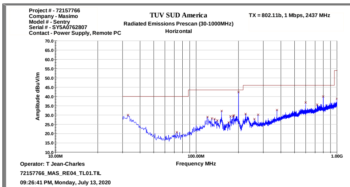
Figure 2.2.7-2: Radiated Emissions Representative Scan 30 MHz – 1 GHz – Horizontal Polarization – Wi-Fi
