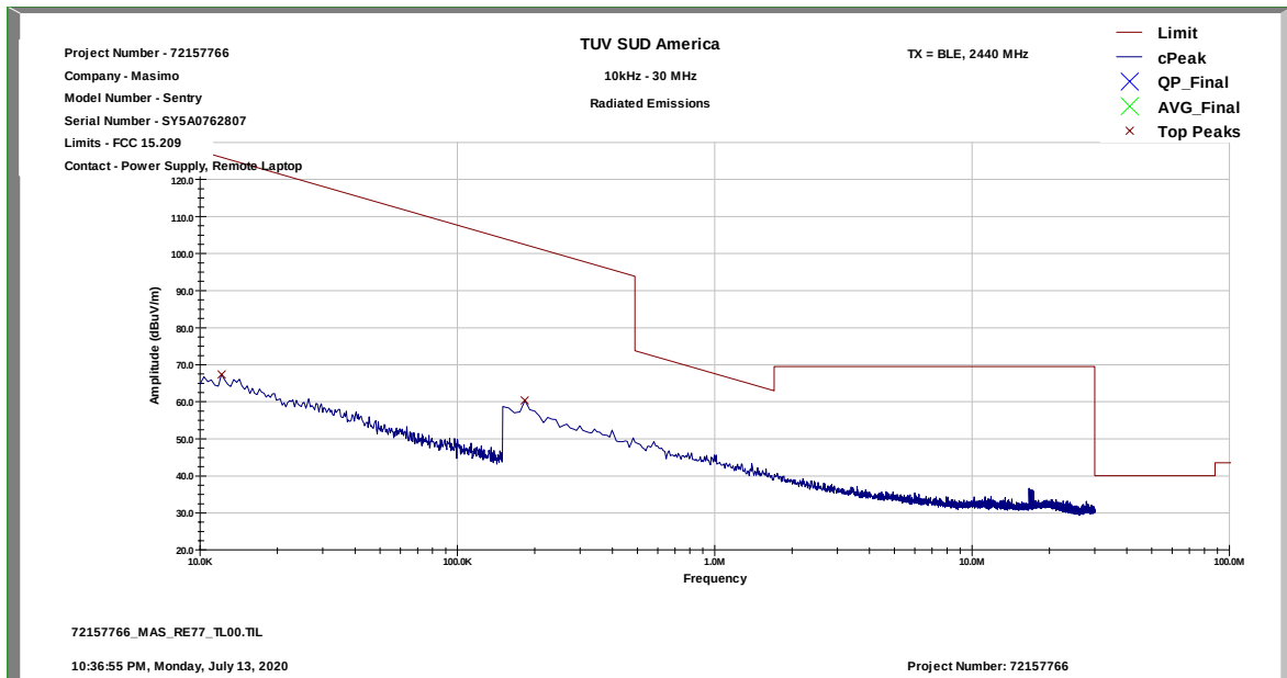
Figure 2.2.7-8: Radiated Emissions Representative Scan below 30 MHz – BLE
