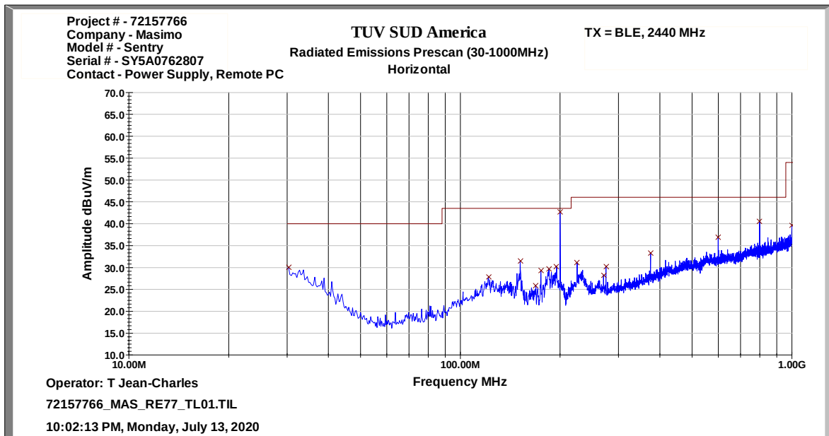
Figure 2.2.7-9: Radiated Emissions Representative Scan 30 MHz – 1 GHz – Horizontal Polarization – BLE
