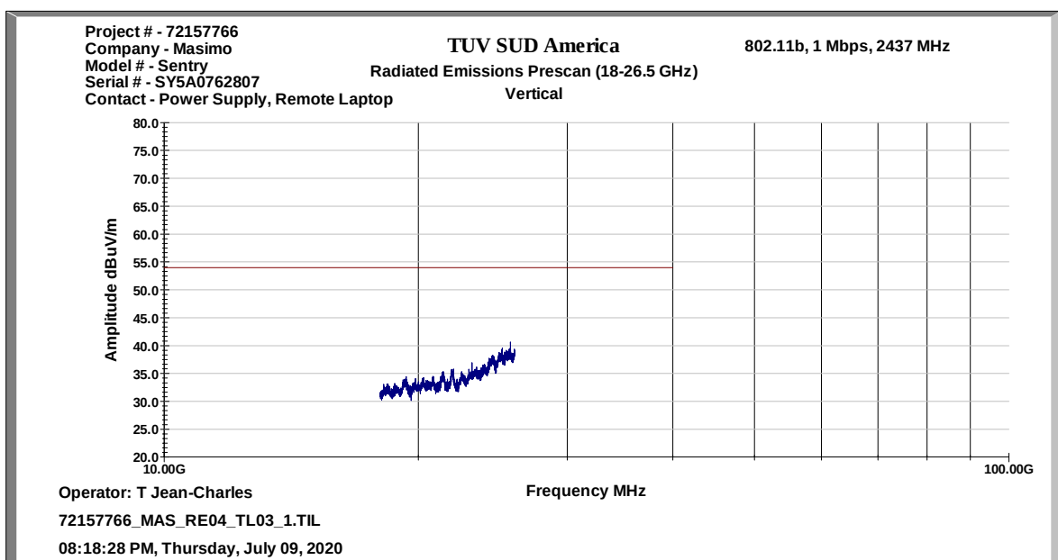
Figure 2.2.7-7: Radiated Emissions Representative Scan 18 GHz – 26 GHz – Vertical Polarization – Wi-Fi
