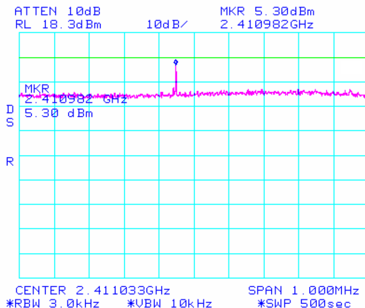
2,412 MHz 802.11b Peak Power Spectral Density
