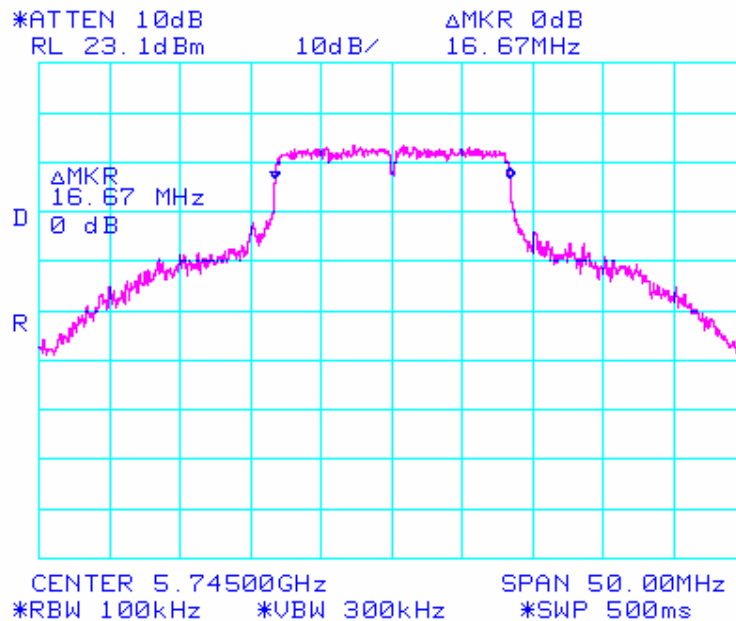
5,745 MHz 802.11a 6 dB Bandwidth
