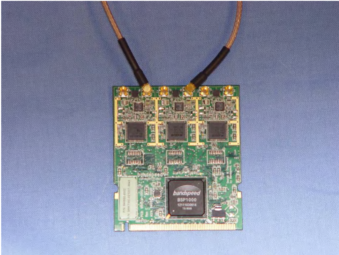
Radio board front
