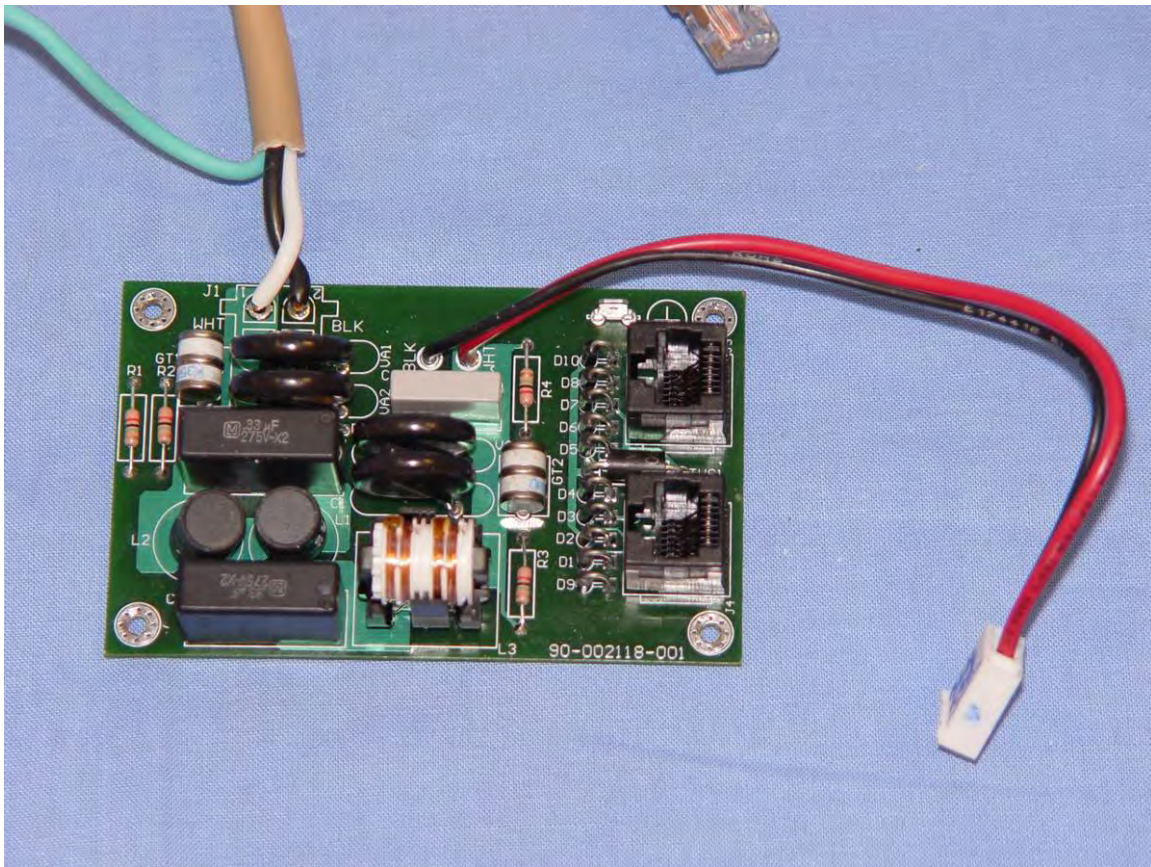
Surge board front
