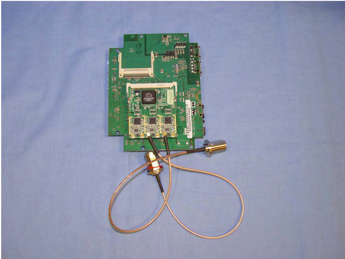
Motherboard with radio board installed
