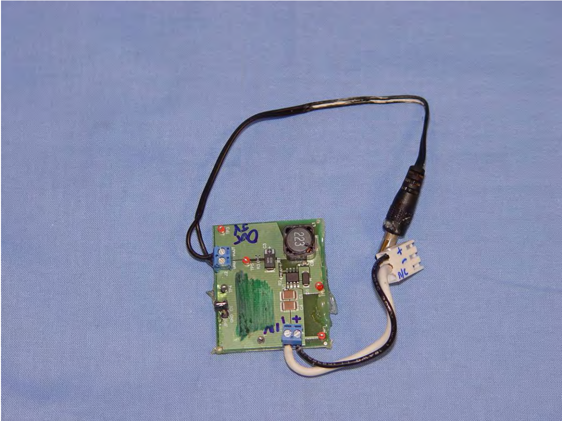
PS aux board front
